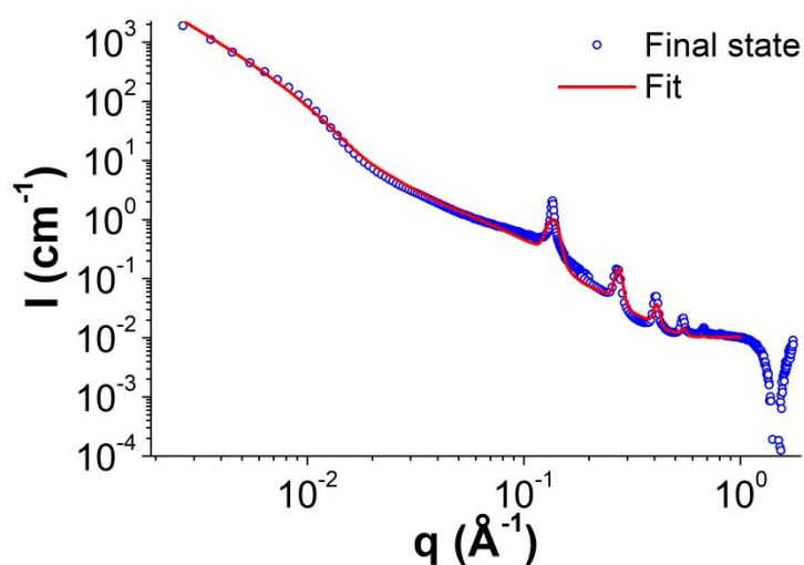
Figure 5: Blue open circles are SAXS-WAXS data for the final state of the \text{Gd}_2\text{O}_2\text{S} nanoparticles obtained with 1.00 equiv. of \text{Na}(\text{oleate}) vs. \text{Gd}(\text{acac})_3 . The solid red line is a best fit using a model of mixed free and aggregated nanoplates (see Supplementary Information).
