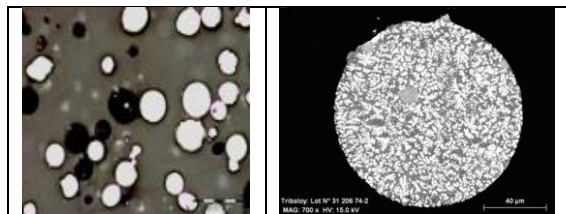
Figure 4: Micrograph of the Tribaloy 700 powder selected in the study (left: global view, right: view of a grain)
