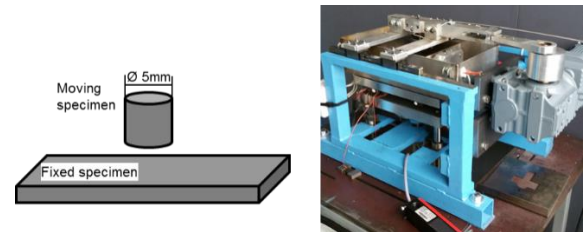
Figure 13: (a) Geometry of sliding wear test and (b) photo of tribometer.
