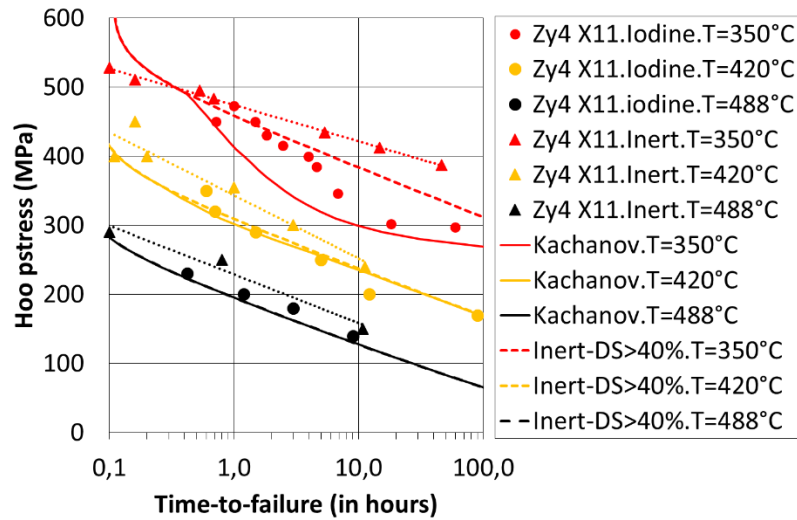
Figure 8 : Inner pressure tests at constant pressure on smooth specimens. Comparison of the Kachanov's model with the experimental results obtained on un-irradiated CWSR Zy-4 (Zy-4 X11 batch) [5].
