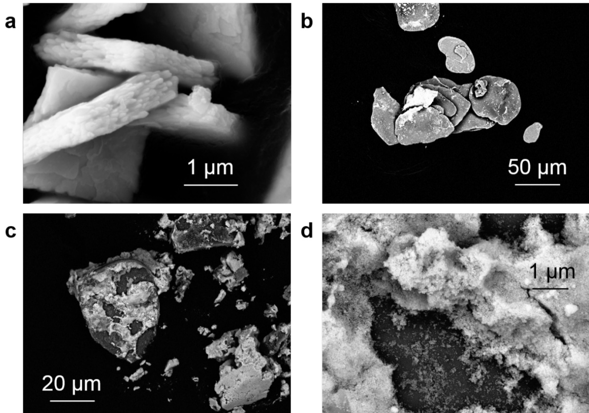
Figure 4: SEM (ETD and BSED) pictures of (a) the initial PuO 2 sample ; (b) sonochemical dissolution residues (20 kHz, 0.45 W mL -1 , Ar, 7 h, 140 mg of Ti 325 mesh, 35 °C) observed for PuO 2 (S BET = 5 m 2 g -1 ) in 1 M HNO 3 /2 M HCOOH/0.1 M HN (V = 50 mL) with the injection of NH 4 F (10 mM) after 180 min of sonication and (c-d) in same conditions except HCOOH is replaced by NHA at 2M. Pu appears in bright colors and Ti in dark.
