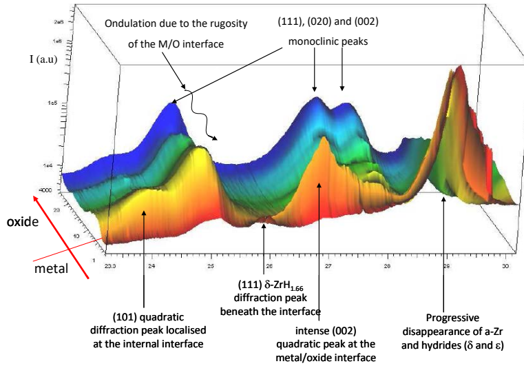
Figure 1 Three dimensional map of \mu -XRD analyses performed on a reference sample corroded in light primary water at 360^{\circ}\text{C} during 171 days (oxide thickness of 3.6\ \mu\text{m} ) [10].
