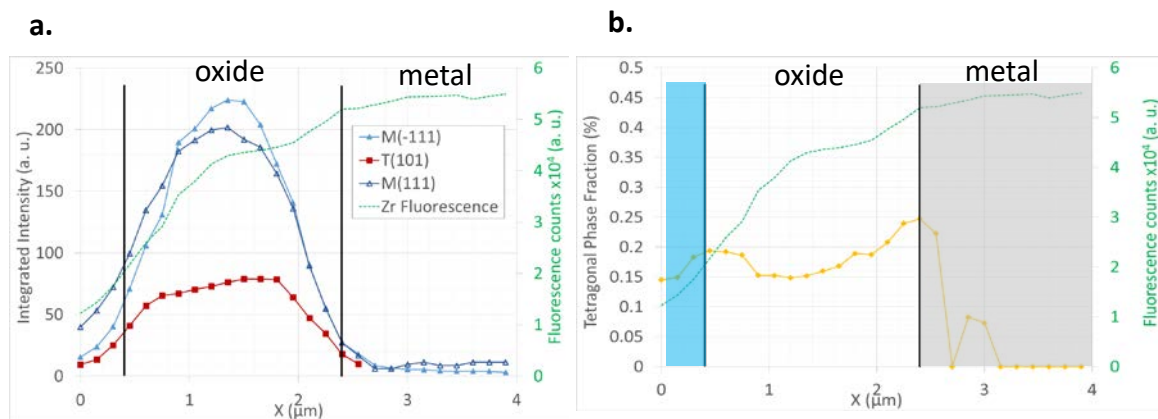
Figure 20 a. Integrated intensity of the monoclinic (111), (\bar{1}11) and the tetragonal (101) oxide peaks; b. tetragonal phase fraction through the thickness of an oxide formed on an irradiated Zircaloy-4 oxide (irradiation conditions: 1.3 MeV He ions, fluence of 10^{17} \text{cm}^{-2} , 0.35 dpa).
