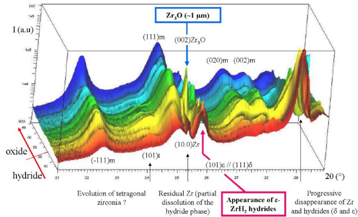
Figure 2 Three dimensional map of \mu -XRD analyses performed on a pre-hydrated sample corroded in light primary water at 360^{\circ}\text{C} (oxide thickness of 7.4\ \mu\text{m} ) [10].
