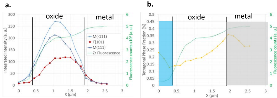
Figure 21 a. Integrated intensity of the monoclinic (111), ( \bar{1}11 ) and the tetragonal (101) oxide peaks; b. tetragonal phase fraction through the thickness of an oxide formed on a sample irradiated Zircaloy-4 oxide then re-oxidized 1 day (irradiation conditions: 1.3 MeV He ions, fluence of 10^{17} cm -2 , 0.35 dpa).
