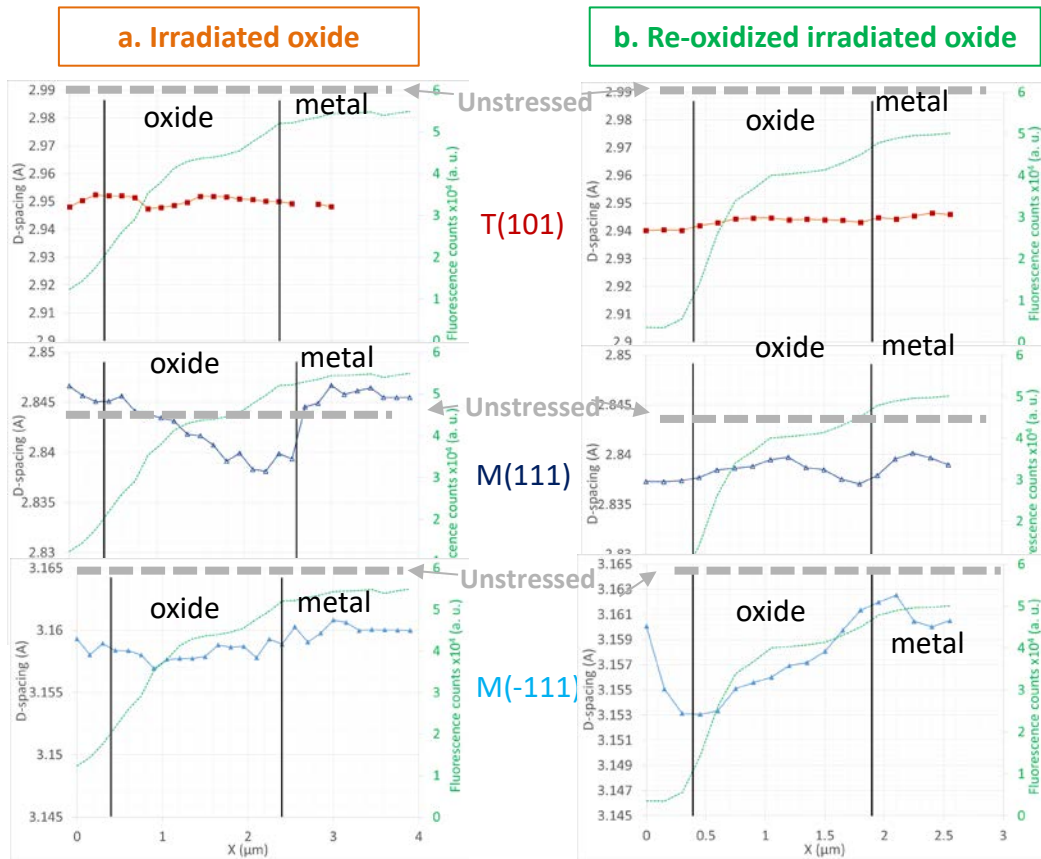
Figure 22 Monoclinic (111), (\bar{1}11) and tetragonal (101) oxide peaks d-spacing through the oxide thickness: a. formed on an irradiated Zircaloy-4 oxide; b. formed on an irradiated Zircaloy-4 oxide then re-oxidized 1 day (irradiation conditions: 300 keV protons, fluence of 10^{18} \text{ cm}^{-2} at 350^\circ\text{C} ).
