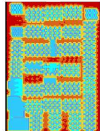
Variance plot
