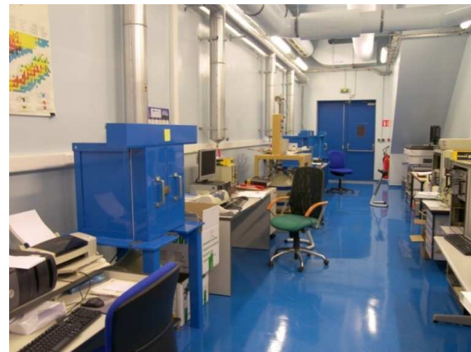
Nuclear analyses
