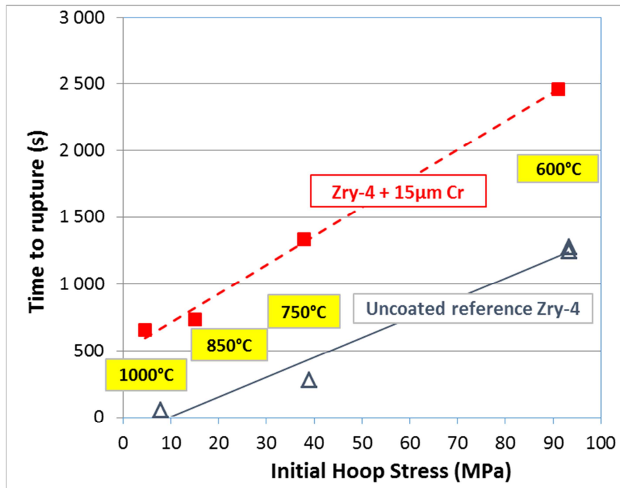
Figure 1 – Time to rupture as a function of the initial hoop stress of uncoated and 15 \mu m thick Cr-coated Zry-4 clad segments for EDGAR (internal pressure) isothermal creep tests performed at different temperatures
