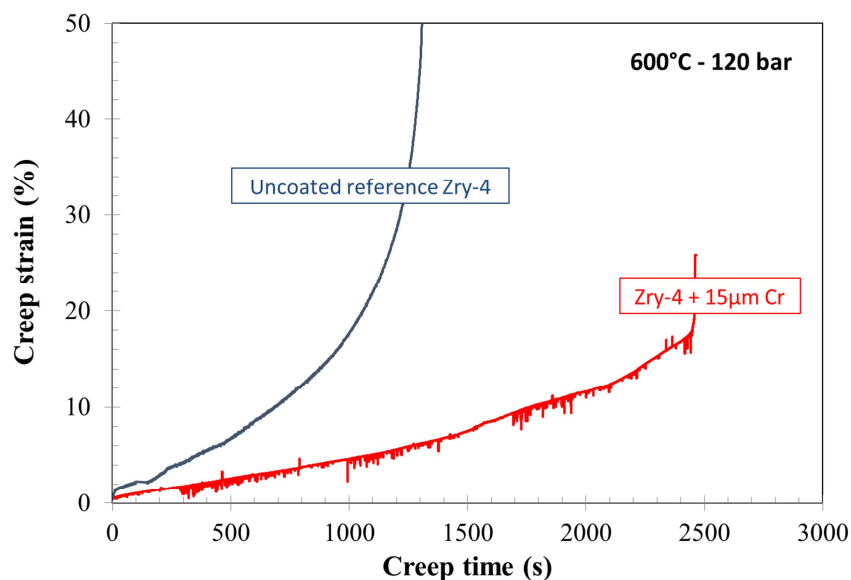
Figure 2 – Typical creep curves obtained on uncoated and 15 \mu m thick Cr-coated Zry-4 clad segments at 600°C, for an applied internal pressure of 120 bar
