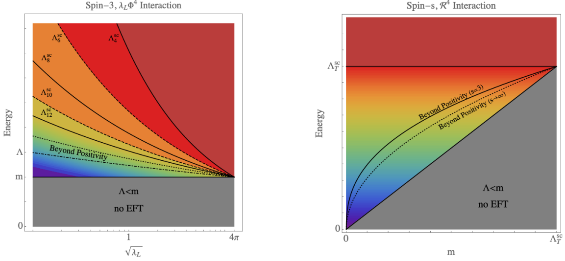
Figure 1. Left: different strong-coupling scales for s = 3 as function of \sqrt{\lambda_L} in eq. (1.31) or eq. (2.23). For E \gtrsim m the interaction strength increases at high energy; the S(V) polarizations are strongly coupled at \Lambda_{12}^{sc}(\Lambda_8^{sc}) generically (solid lines) or at \Lambda_{10}^{sc}(\Lambda_6^{sc}) for the tuned theory (dashed lines). Beyond-positivity bounds for the \lambda_L \Phi^4 interaction (dotted) and \lambda_L \partial^4 \Phi^4 / \Lambda^4 (dot-dashed): this represents the maximal cutoff \Lambda of the theory, well below the strong-coupling scales. Right: similar energy scales and beyond-positivity bounds for the \mathcal{R}^4 interaction as function of m (solid line for s=3 , dotted for s \rightarrow \infty ).
