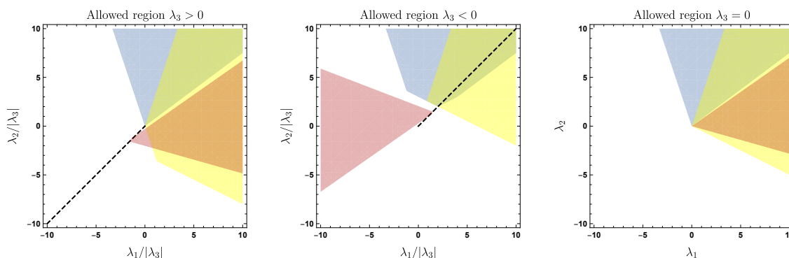
Figure 2. Allowed regions of the coefficients \lambda_1, \lambda_2 as function of the sign of \lambda_3 . Blue: result from scattering of linear-definite polarizations eq. (2.31). Red: result from \Sigma_{\text{IR}}^{(2)} > 0 by scattering different choices of linear combination of polarizations. Yellow: result from \Sigma_{\text{IR}}^{(4)} > 0 by scattering only linear-definite polarizations. The dotted line correspond to the tuning \lambda_1 = \lambda_2 = -\lambda_3 in eq. (2.8).
