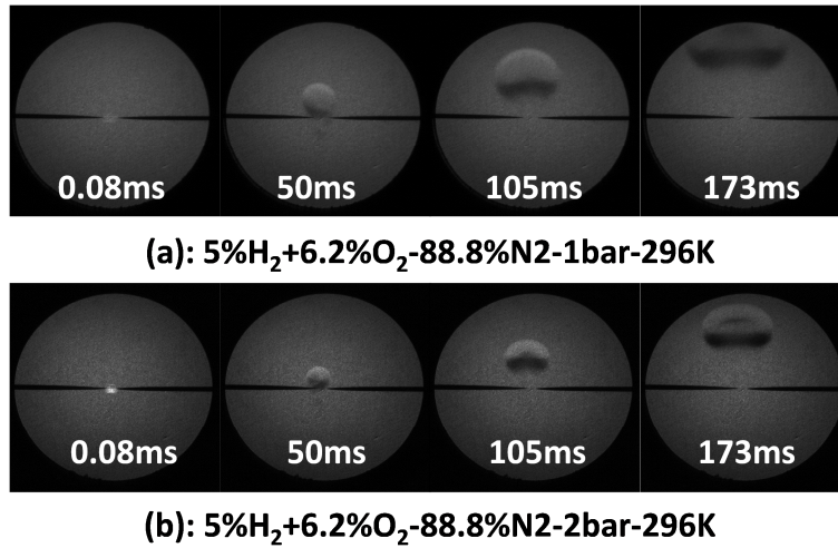
Figure 10 Typical flame propagation regimes for H_2/O_2/N_2 mixtures close to the flammability limit. (a): 1 bar and 296 K; (b): 2 bar and 296 K
