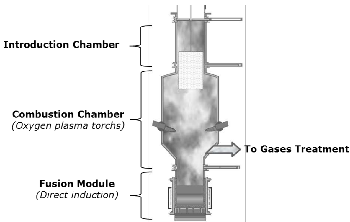
Fig. 2. Heart of the PIVIC process schematic diagram.
