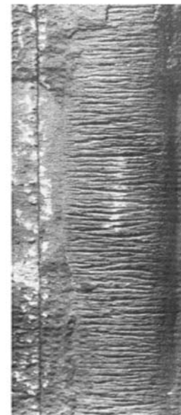
Supercritical waterwall cracking, from Steag, 2013, http://www.eecpowerindia.com/codelibrary/ckeditor/userfiles/files/Water_Quality_for_Supercritical_Units_steag_for_mat.pdf
