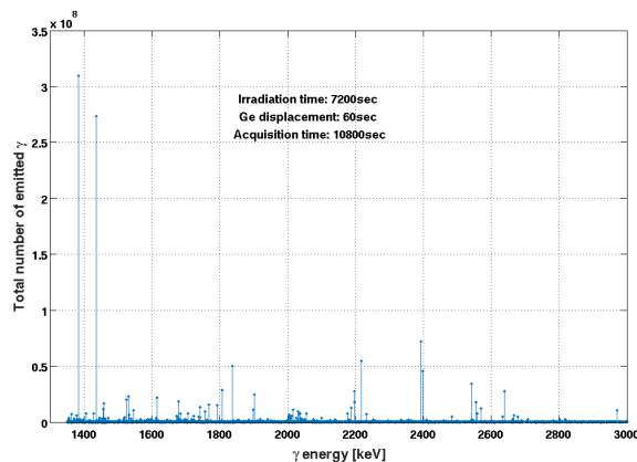
Fig. 5. Delayed \gamma spectrum for ^{235}\text{U} photofissions integrated over the acquisition time.
