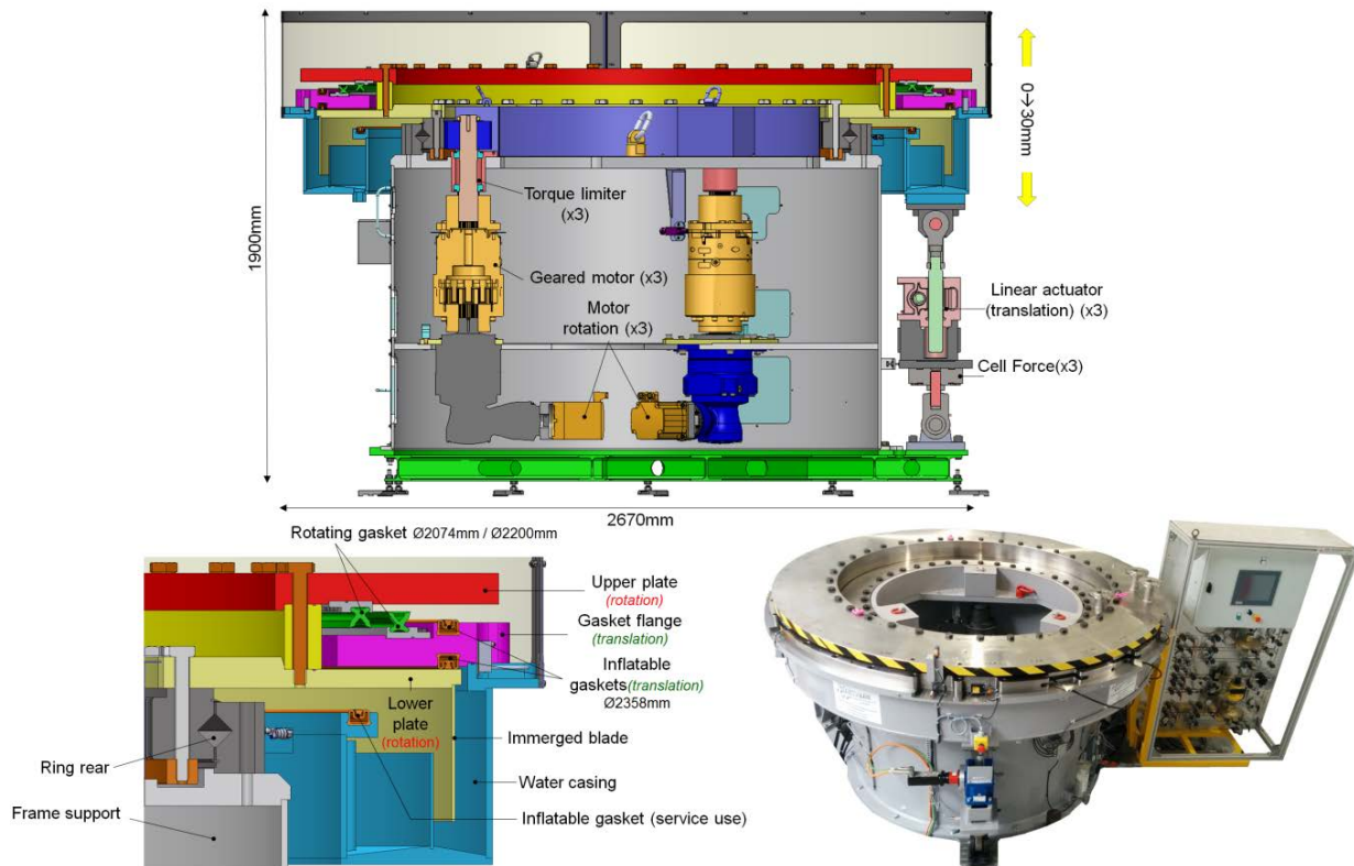
FIG. 1. Top: RST schematic cut-view of the mechanical structure; Bottom left: detailed cut-view; Bottom right: picture of the RST
