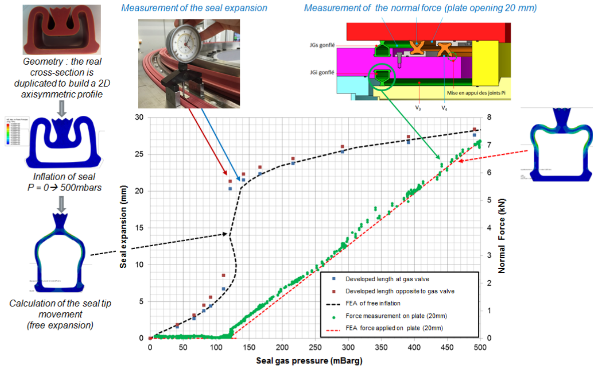
FIG. 4. Inflatable seal comparison between experimental measurements and FEA: FEA results - dashed lines, experimental measurements - dots
