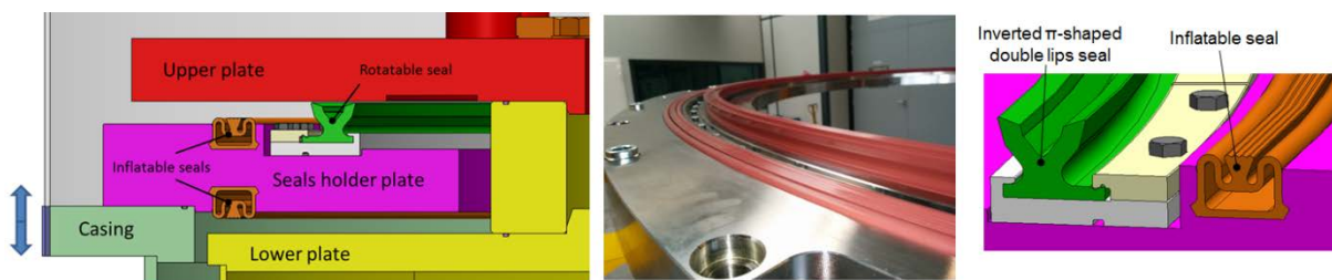
FIG. 3. Assembly of the inflatable and inverted- \pi shaped seals on the RST
