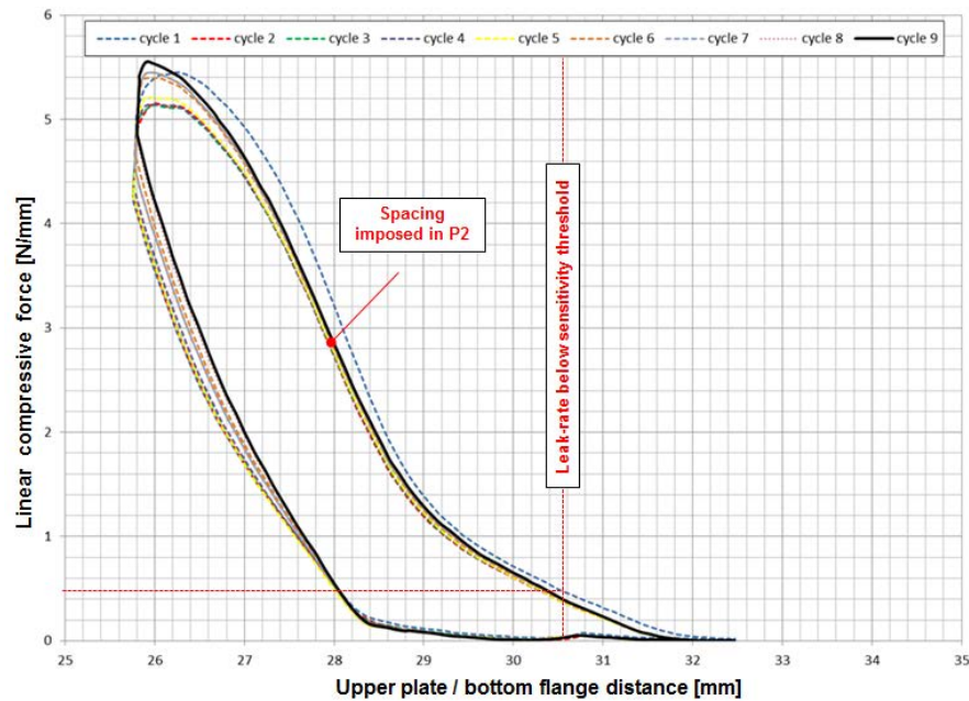
FIG. 5. Compression curves of the Rotatable inverted- \pi shape seal: linear compressive force as a function of plates spacing (the last cycle is in bolded line).
