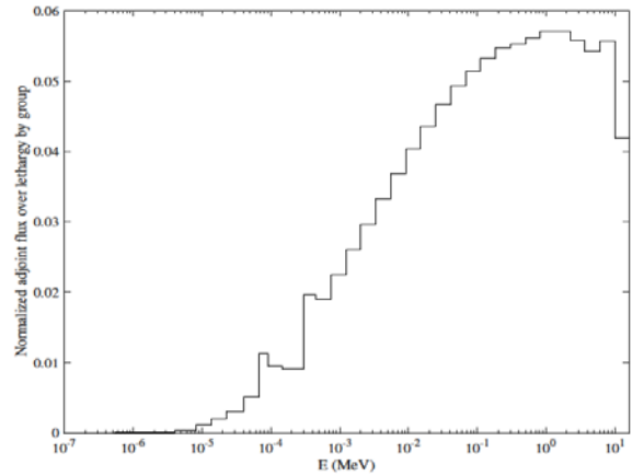
Fig. 8. Adjoint flux in the center – ERANOS calculation
