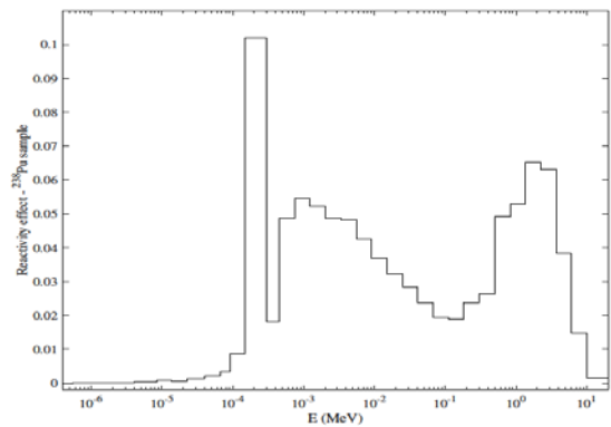
Fig. 11. \Delta\rho energy distribution due to a ^{238}\text{Pu} sample (in pcm)
