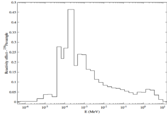
Fig. 10. \Delta\rho energy distribution due to a ^{239}\text{Pu} sample (in pcm)
