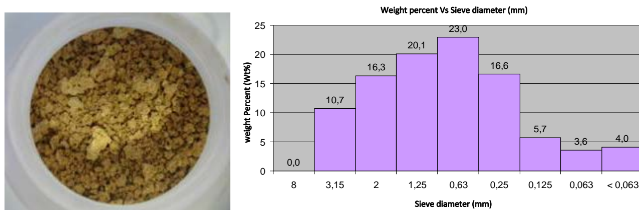
Fig. 4. Calcine obtained with the appropriate adjustment and operating parameters
