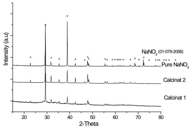
Fig. 6. X-ray diffraction diagrams of calcines 1, 2 and \text{NaNO}_3
