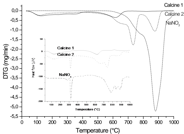
Fig. 7. Differential thermal and thermogravimetric analyses of calcine samples and \text{NaNO}_3 pure phase
