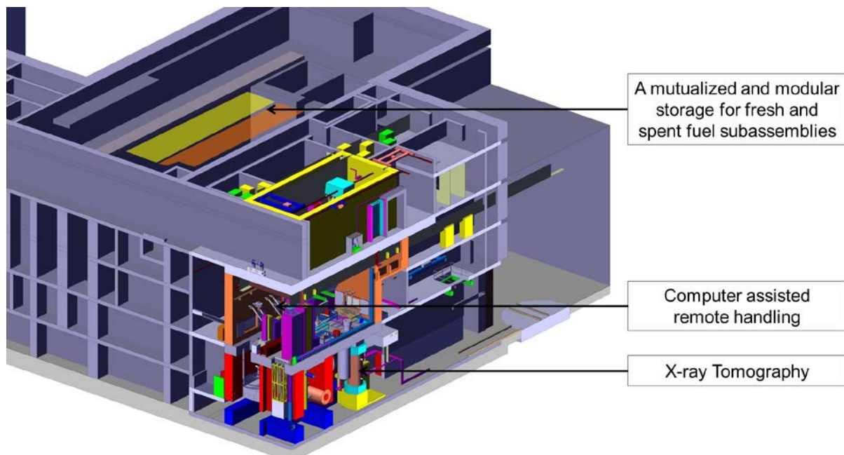
FIG. 3. - Innovations location in fuel handling building
