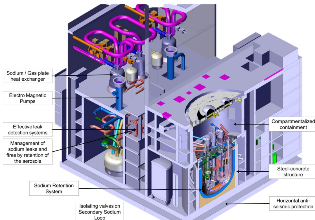
FIG. 2. - Innovations location in the nuclear island
