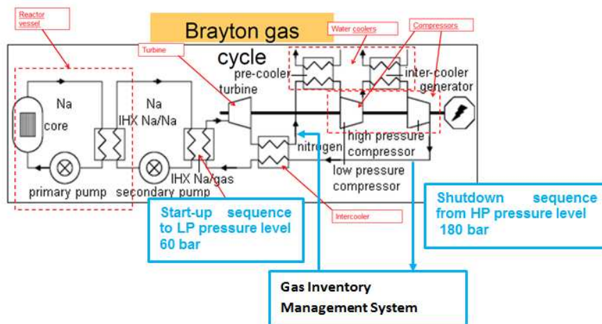
FIG 4: Scheme of gas inventory management system
