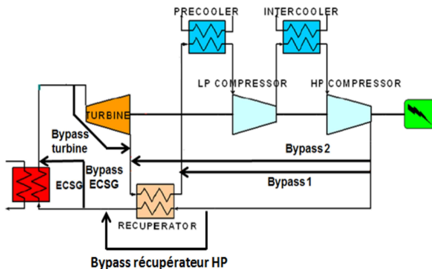
FIG.2: Scheme of several by passes tested on Brayton cycle
