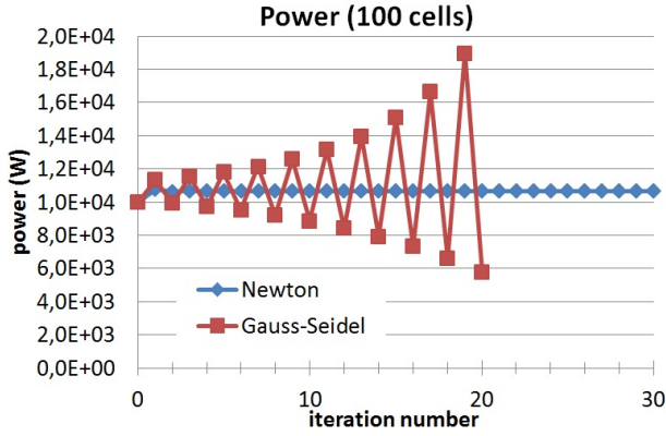
Fig. 3. Global power from different coupling techniques, with 100 cells.
