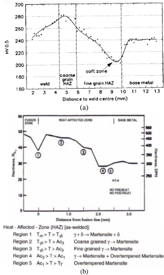
Figure 9: (a) hardness profile after PWHT through a P91 welded joint [5], (b) correlation between welded microstructure, maximum temperature and hardness value [7]
