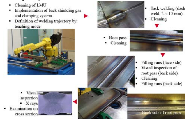
Figure 7: main welding steps on LMU
