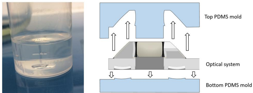
Figure 9: Photography of the mother molded in PDMS (left). Cross sectional view of the unloading step (right)
