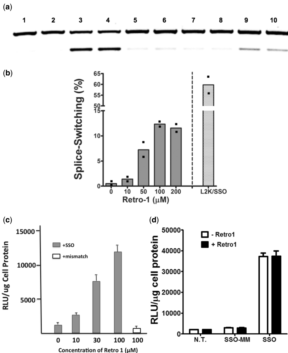
Figure 3. Retro-1 effects on the splicing of an endogenous RNA and exploration of mechanisms. (a) Retro-1 enhances SSO effects on an endogenous message. PC3 cells were treated for 16 h with 250 nM of an SSO that shifts the splicing of Bcl-x pre-mRNA to the Bcl-x S form. Cells were subsequently treated with 100 μM Retro-1 for 2 h or maintained as controls. Cells treated with the SSO complexed with Lipofectamine 2000 provided a positive control. RNA was extracted and analysed by RT-PCR as described in 'Materials and Methods' section. Upper band, Bcl-x L product; lower band, Bcl-x S product. Lanes 1,2 untreated control (no SSO); Lanes 3,4 SSO + Lipofectamine 2000; Lanes 5,6 SSO only; Lanes 7,8 Retro-1 only; Lanes 9,10 SSO + Retro-1. (b) Dose-response for Bcl-x splicing modification. In an experiment similar to that of Figure 3a, various concentrations of Retro-1 were tested. Band intensities were quantitated with a gel scanner as described in 'Materials and Methods' section. The ordinate shows the ratio of the Bcl-x S (lower) band to the total (upper plus lower) band intensity expressed as a percentage. Bars show mean values, individual values shown as black squares. n = 2. (c) Retro-1 treatment does not cause non-specific increases in splicing activity. A375Luc705 cells were incubated with 50 nM SSO 623 or its mismatch control. After removal of the oligonucleotide, the cells were treated (2 h) with various concentrations of Retro-1. After removal of the Retro compound and further incubation, luciferase activity and cell protein were measured. Grey bars, SSO 623; open bar, mismatch oligonucleotide. n = 6. Mean + standard error. (d) Retro-1 does not affect the action of oligonucleotides delivered by electroporation. SSO 623 or its mismatch control (SSO-MM) (100 pmoles) were directly delivered to the cytosol of A375Luc705 cells by Amaxa ® electroporation. Thereafter, the cells were treated for 2 h with Retro-1 (100 μM). After removal of the Retro compound, the cells were further incubated and then assayed for luciferase activity and cell protein. Black bar, +Retro-1; white bar, - Retro-1; NT, not treated. n = 3. Mean + standard error.
