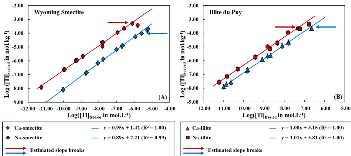
Fig. 2. Results in \log([Tl]_{\text{sorbed}}) = f([Tl]_{\text{free,eq}}) for smectite (A) and illite (B). Error bars correspond to the variability of Tl sorbed. pH condition are 7.34 \pm 0.40 , 7.89 \pm 0.20 , 5.00 \pm 0.10 and 7.18 \pm 0.08 for respectively Na-smectite, Ca-smectite, Na-illite and Ca-illite (Figs. 3B, 4B, 5B and 6B captions).
