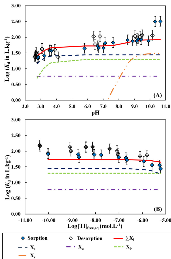
Fig. 4. Results for Ca-smectite in \log K_d = f(\text{pH}) (A) and in \log K_d = f([\text{Tl}]_{\text{free,eq}}) (B). In A, introduced average Tl concentration, [\text{Tl}]_{t=0} = 2.12 \pm 0.29 \cdot 10^{-10} \text{ mol L}^{-1} . In B, sorption average pH was 7.89 \pm 0.20 and was 7.97 \pm 0.04 during desorption. Dashed colorful lines correspond to contribution of individual modeled reactive sites. Red lines are the sum of each site contribution. Error bars correspond to the K_d variability. (For interpretation of the references to colour in this figure legend, the reader is referred to the web version of this article.)
