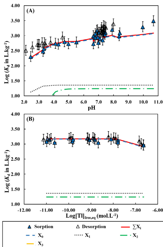
Fig. 6. Results for Ca-illite in \log K_d = f(\text{pH}) (A) and in \log K_d = f([\text{Tl}]_{\text{free,eq}}) (B). In A, introduced average Tl concentration, [\text{Tl}]_{i=0} = 4.37 \pm 0.18 \cdot 10^{-8} \text{ mol L}^{-1} . In B, sorption average pH was 7.18 \pm 0.08 and was 7.14 \pm 0.19 during desorption. Dashed colorful lines correspond to \log K_d for each modeled reactive sites. Red lines are the sum of each site contribution. Error bars correspond to the K_d variability. (For interpretation of the references to colour in this figure legend, the reader is referred to the web version of this article.)
