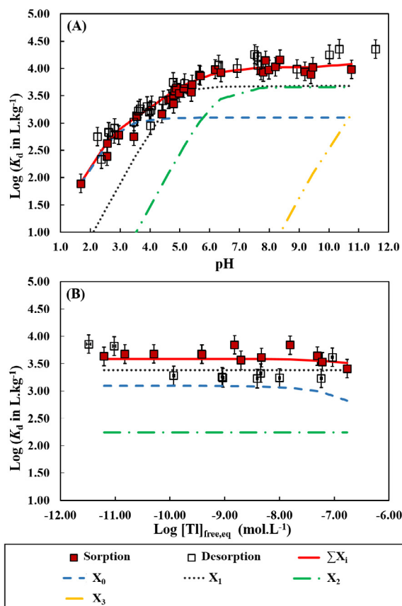
Fig. 5. Results for Na-illite in \log K_d = f(\text{pH}) (A) and ion \log K_d = f([\text{Tl}]_{\text{free,eq}}) (B). In A, introduced average Tl concentration, [\text{Tl}]_{i=0} = 4.01 \pm 0.95 \cdot 10^{-8} \text{ mol L}^{-1} . In B, sorption average pH was 5.00 \pm 0.10 . For desorption, it was 5.00 \pm 0.46 for points with \log [\text{Tl}]_{\text{free,eq}} < -10 \text{ mol L}^{-1} and for the point (-7.03; 3.62) . Then, it was 3.94 \pm 0.19 for points with \log [\text{Tl}]_{\text{free,eq}} > -10 \text{ mol L}^{-1} . Dashed colorful lines correspond to contributions of individual modeled reactive sites. Red lines are the sum of each sites. Error bars correspond to the variability of the K_d . (For interpretation of the references to colour in this figure legend, the reader is referred to the web version of this article.)
