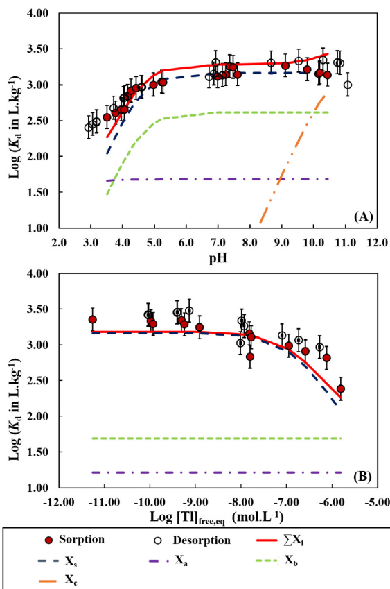
Fig. 3. Results for Na-smectite in \log K_d = f(\text{pH}) (A) and in \log K_d = f([\text{Tl}]_{\text{free,eq}}) (B). In A, introduced average Tl concentration is [\text{Tl}]_{t=0} = 2.24 \pm 0.08 \cdot 10^{-10} \text{ mol L}^{-1} . In B, sorption average pH was 7.34 \pm 0.40 and was 6.11 \pm 0.40 during desorption. Dashed colorful lines correspond to the individual modeled reactive sites contributions. Red lines are the sum of each site contribution. Error bars correspond to the K_d variability. (For interpretation of the references to colour in this figure legend, the reader is referred to the web version of this article.)
