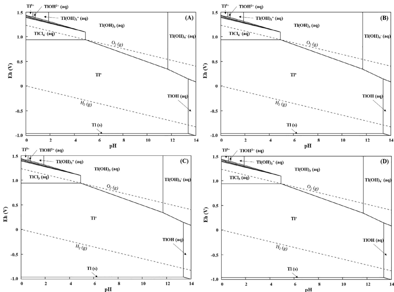
Fig. 1. Eh-pH diagrams for thallium. A Tl-Ca-Cl-H 2 O system is described for A and B with [CaCl 2 ] = 10 mM. In A, [Tl] = 100 nM and in B, [Tl] = 0.1 nM. C and D describe a Tl-Na-Cl-H 2 O system with [NaCl] = 10 mM and [Tl] = 100 nM for C and 0.1 nM for D. Tl constants database is from Casiot et al. (2011) except for TlOH(aq) which is calculated from Brown and Ekberg's book (2016). Diagrams made with JChess v2.0.
