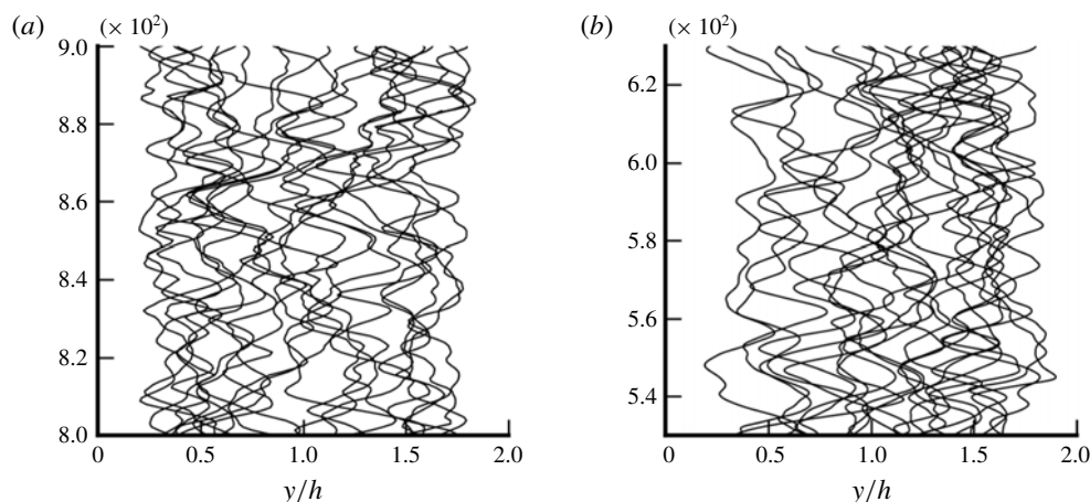
FIGURE 7. Wall-normal positions of the 21 large bubbles in case D (a); and in case B (b); on a time interval of 100 s.
