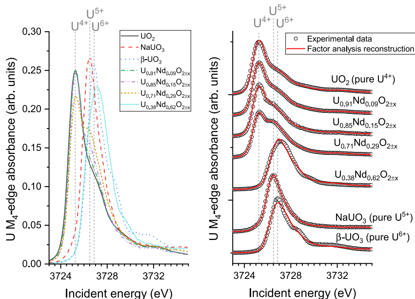
Fig. 2. (Left) Uranium M 4 -edge HERFD-XANES experimental spectra recorded on UO 2 , NaUO 3 , β-UO 3 and U y Nd 1-y O 2±x collected at ID26. The X-ray emission spectrometer was tuned to the maximum energy of the M β emission line. (right) Experimental (open symbols) and reconstructed spectra from factor analysis (full lines). Spectra were vertically shifted for sake of clarity.
