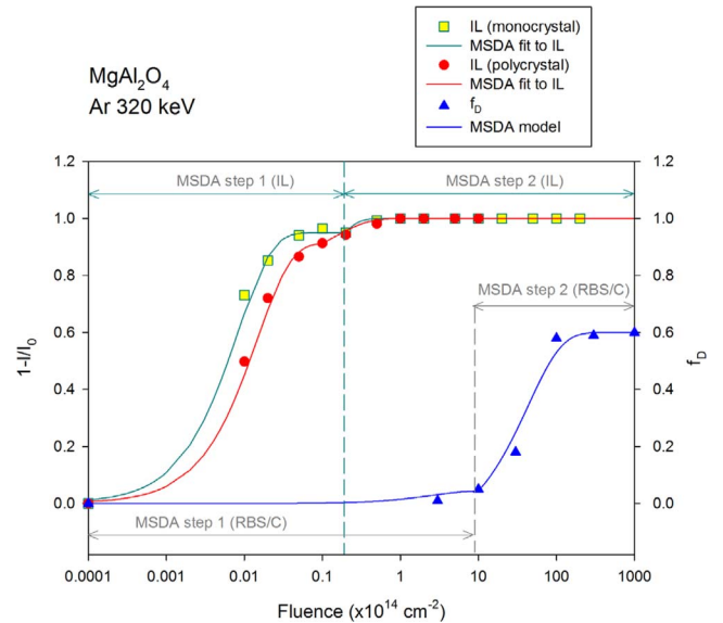
Fig. 3. Damage accumulation kinetics in MgAl 2 O 4 irradiated with 320 keV Ar + ions calculated from: RBS/C data (triangles) and ionoluminescence data (circles and squares). Lines are fits with the MSDA model assuming a two-step process.
