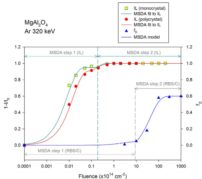
Fig. 3. Damage accumulation kinetics in MgAl 2 O 4 irradiated with 320 keV Ar + ions calculated from: RBS/C data (triangles) and ionoluminescence data (circles and squares). Lines are fits with the MSDA model assuming a two-step process.
