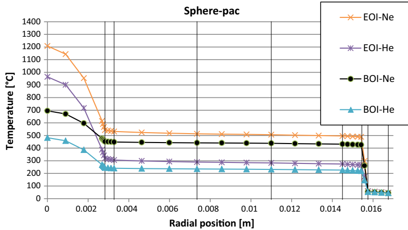
Fig. 23. Comparison of radial temperature distribution for the different load cases, sphere-pac.
