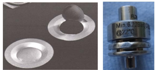
Fig. 13. The burst disks on the left and within its holder on the right.
