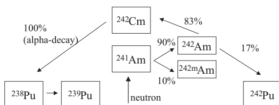
Fig. 1. Reaction chain of 241 Am.
