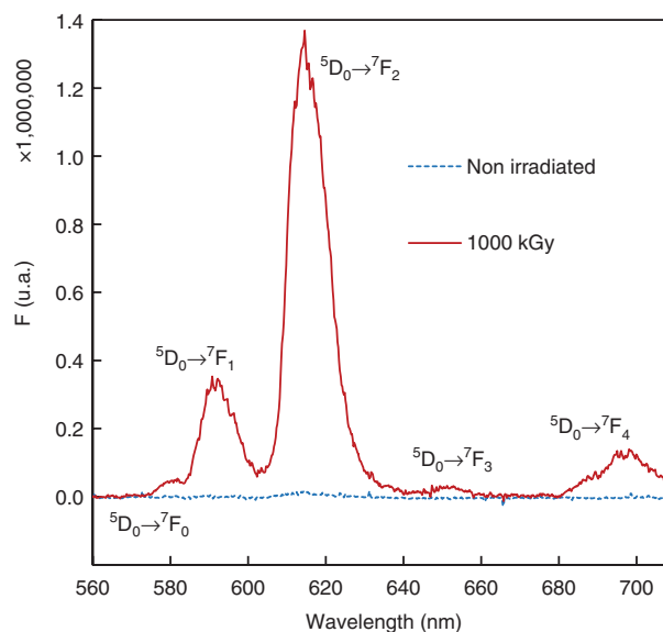
Figure 2: Luminescence spectra of Eu(III) in solution with HDPs from non-irradiated PURE (dotted line) and \gamma -PURE (plain line) in SACPW: [\text{Eu}] = 10^{-6} \text{ mol} \cdot \text{kg}_w^{-1} ; D = 10 \mu\text{s} , W = 300 \mu\text{s} , \lambda_{\text{exc}} = 393.8 \text{ nm} . HDPs are released after the leaching of the polymer in the SACPW solution for one month at 60 °C. HDPs were diluted by two to obtain these spectra.
