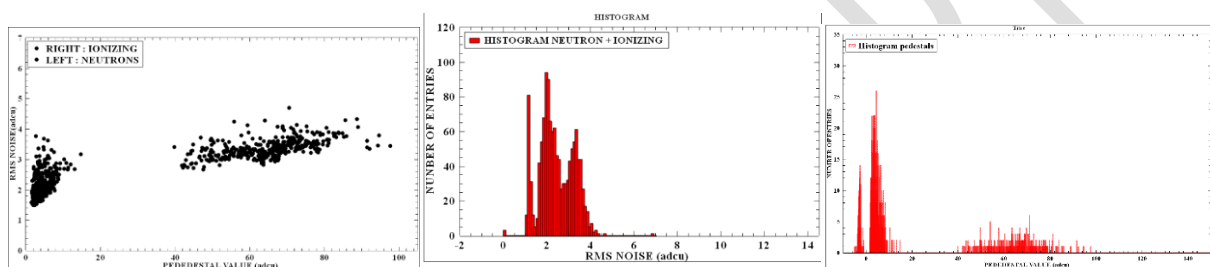
Fig.22: Temporal noise versus offset (pedestal), neutron on the left side and ionizing right side. The others are histograms for the rms noise and pedestals (ref 64) [23].
