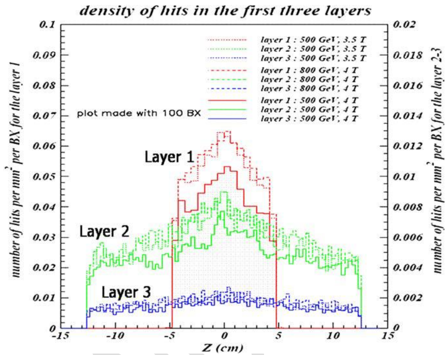
Fig.15: number of hits per bunch crossing/ squared mm 2 in three layers plotted versus the Z (incident beam) directions for the ILC [49].
