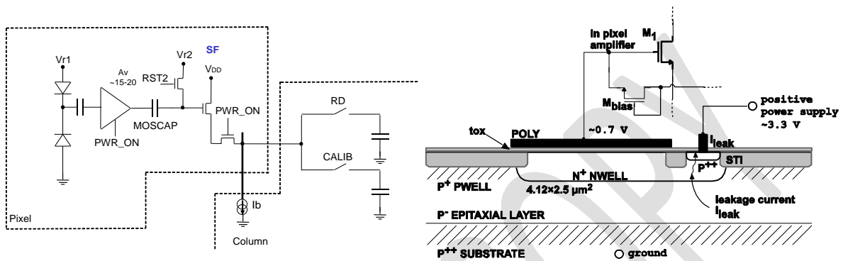
Fig.5. Pixel configurations and schematics of the MIMOSA series (MIMOSA 6).The sensitive part is the photodiode [44] [26].
