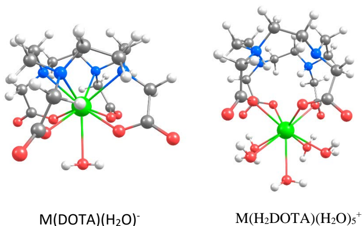
Figure 10. Schematic representation of M(\text{DOTA})(\text{H}_2\text{O})^- and M(\text{H}_2\text{DOTA})(\text{H}_2\text{O})_5^+ complexes.
