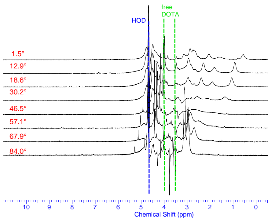
Figure 6: 1 H NMR spectra of 0.1M DOTA in D 2 O with Pu(III) at different temperatures. [DOTA]/[Pu]=5 and pH=2. The pulse sequence used (WET1D) eliminated water and the free DOTA signals.
