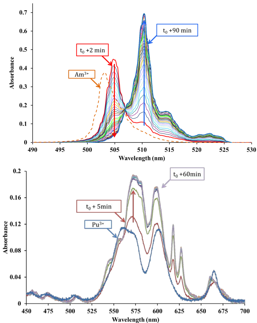
Figure 2. top: UV-Vis kinetic follow-up of the complexation of 10^{-3}\text{M Am}^{3+} by 0.1\text{M DOTA} in aqueous solution at \text{pH} = 3.5 \pm 0.3 and \theta = 25^\circ\text{C} . Dashed orange line: \text{Am}^{3+} 10^{-3}\text{M} in 0.1\text{M HNO}_3 . t_0 : addition of the metal solution to the ligand solution. Bottom: UV-Vis kinetic follow-up of the complexation of 3.6 \cdot 10^{-3}\text{M Pu}^{3+} by 0.2\text{M DOTA} in aqueous solution at \text{pH} = 3.5 \pm 0.3 and \theta = 25^\circ\text{C} . Blue line: 2 \cdot 10^{-3}\text{M Pu}^{3+} in 1\text{M HCl} , 0.14\text{M ClHA} .
