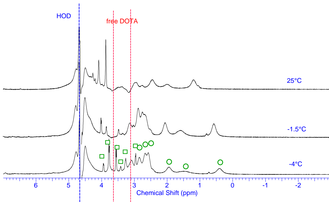
Figure 7: 1 H NMR spectra of 0.1M DOTA in D 2 O with Pu(III) without (bottom one) and with water and free DOTA signal suppression (WET1D pulse sequence) to enhance resolution of the DOTA complex signals. Assignments of two isomer complexes are pointed with circle and square green tags at -4°C.
