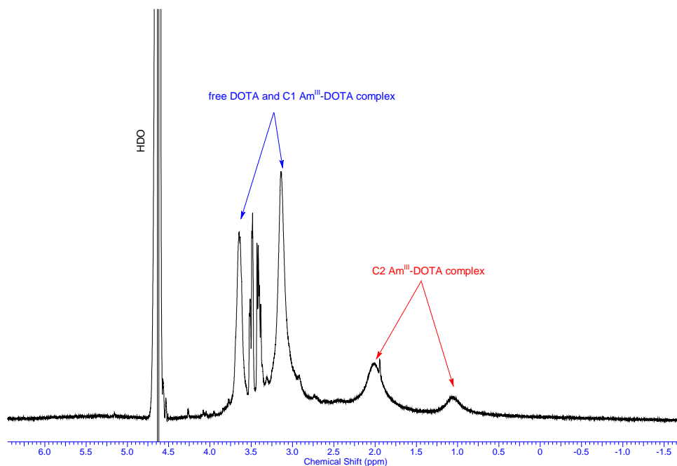
Figure 9: ^1\text{H} NMR spectrum of 0.1M DOTA in \text{D}_2\text{O} with \text{Am}^{\text{III}} nitrate. [\text{DOTA}]/[\text{Am}^{\text{III}}]=2 and \text{pH}=2.7 .
