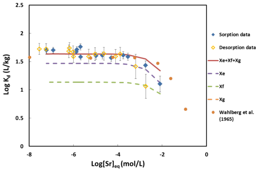
Fig. 4. (a) and (b) Logarithm of the Sr distribution coefficient vs. pH (a) ( [Sr]_i = 10^{-7}M ) and vs. the Sr concentration at equilibrium on Ca-smectite ( I=0.03M ) (pH=7.5 (here, blue diamonds for sorption and yellow for desorption) and pH=7 (Wahlberg et al. (1965) (orange dots)) and (b) the modeling outcome (red line). Contribution of the high-capacity sites Xe, Xf and Xg (violet, green and orange dashed lines).
