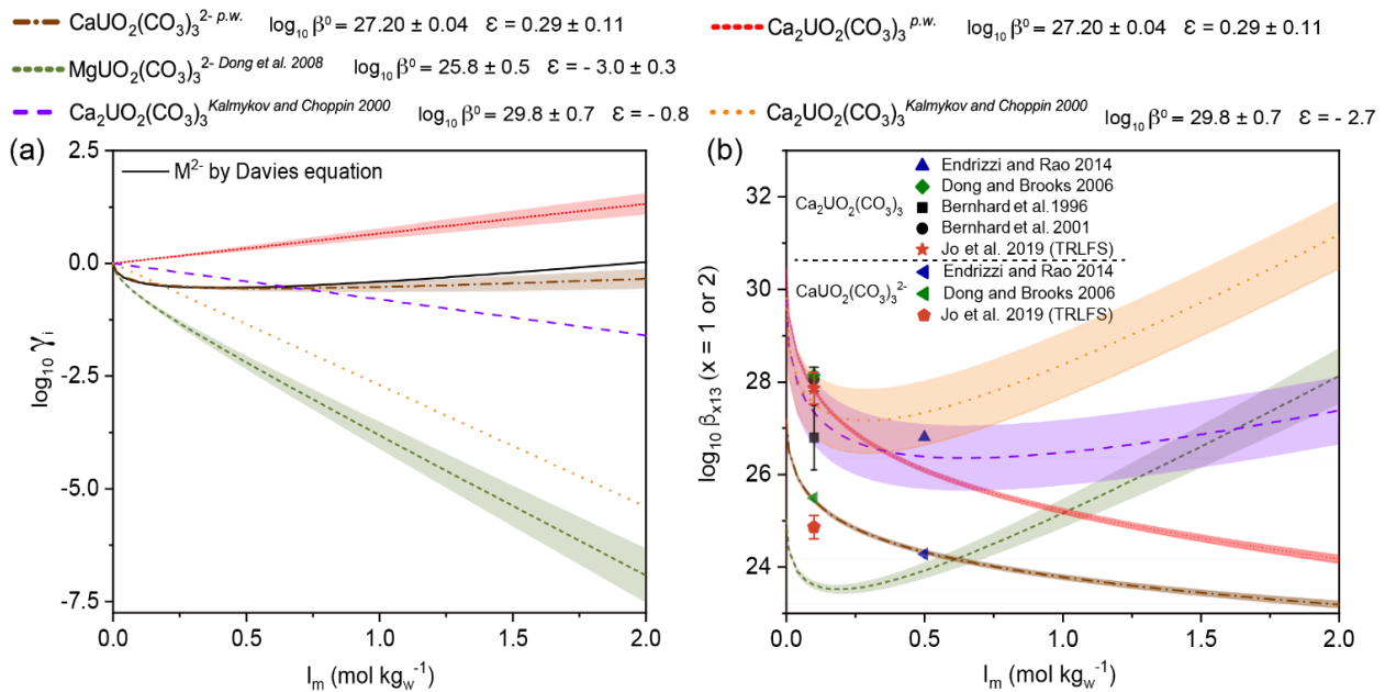
Figure 7. Variations of activity coefficients (a) and formation constants (b) for the M_n UO 2 (CO 3 ) 3 (4-2n)- complexes (M being Mg or Ca) as a function of molal ionic strength.
