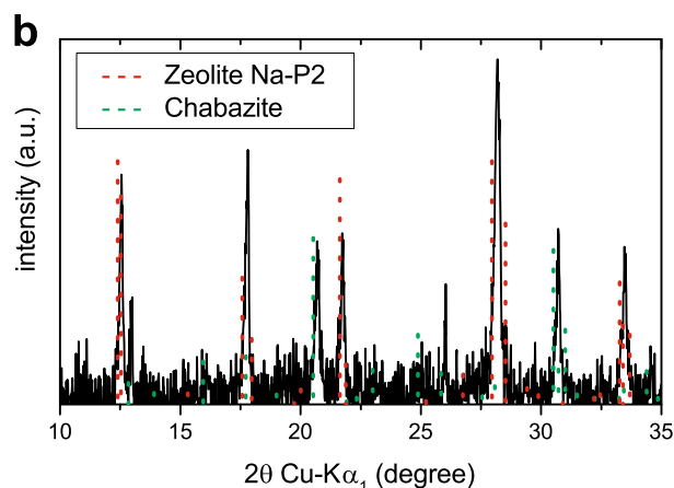
Fig. 5 Seeds growth at 90 °C, pH = 10.1. a At pH_{90\text{ °C}} = 10.1 , two crystals with very different morphologies are observed (seeds of Na-P2 zeolite indicated by the red arrow and neoformed crystals indicated by the green arrow). Scale bar represents 10 \mu\text{m} . b XRD identified Na-P2 zeolite (JCPDS 80-0700), introduced as seeds, which supports the growth of another zeolite: chabazite (JCPDS 34-0137). The background was subtracted for readability
