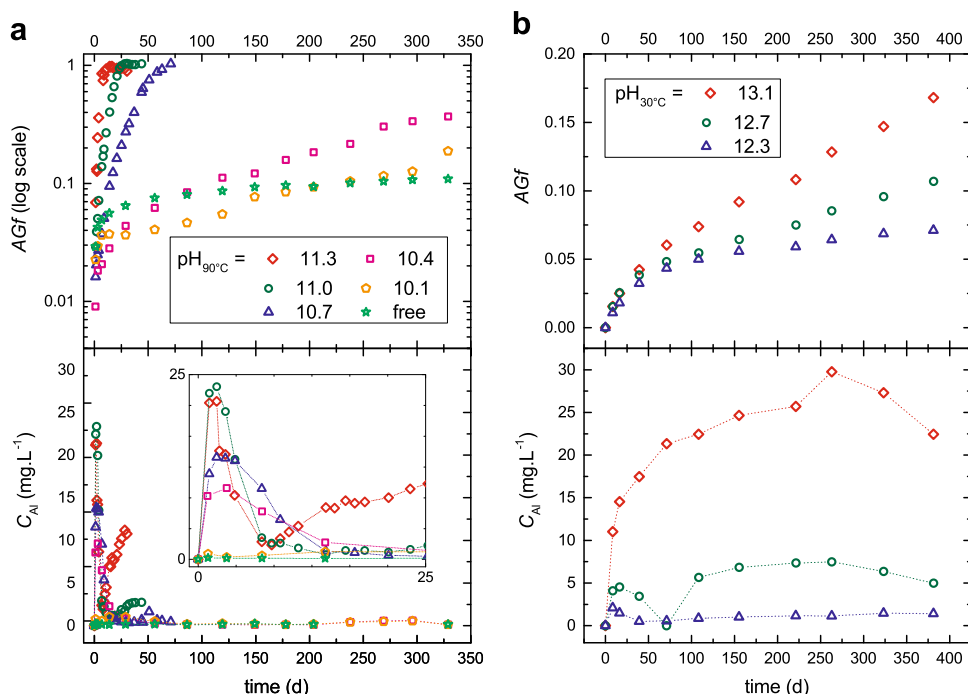
Fig. 3 Seeded leaching tests results: at a 90 °C (S-1770 test series) and b 30 °C (s-1770 test series) with an S/V ratio of 1770 m -1 . Graphs show the evolution of the altered glass fraction AGf and the aluminum concentration. Figure to compare with Fig. 1 for unseeded tests
