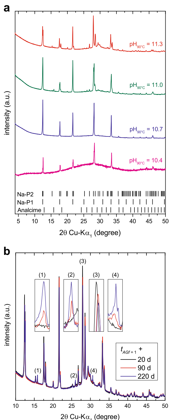
Fig. 2 Secondary phases identification. a X-ray diffraction patterns for tests performed at 90 °C with an S/V ratio of 1770 m -1 (test series US-1770). The identified phases are zeolite Na-P2 (JCPDS 80-0700), zeolite Na-P1 (JCPDS 71-0962) and analcime (JCPDS 76-0904). b X-ray diffraction patterns of crystalline phases formed 20, 90 and 220 days after achieving complete glass alteration ( t_{AGf} = 1 ) at 90 °C and S/V = 1770 m -1 . Peaks 1, 2, and 4 on which are performed the magnifications correspond to the major peaks of analcime: it becomes more intense as the peaks of the zeolites P become less intense (peak 3)
