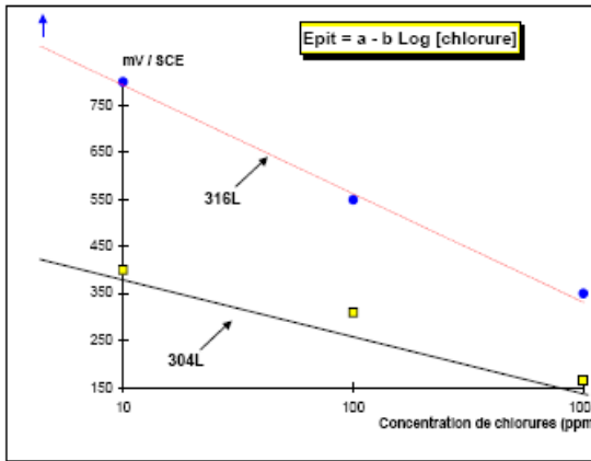
Pitting potential
