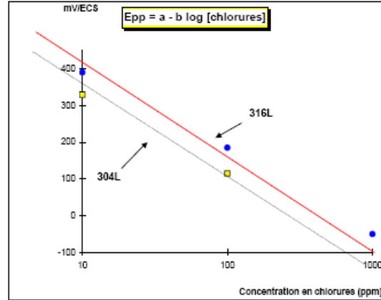
Repassivation potential
