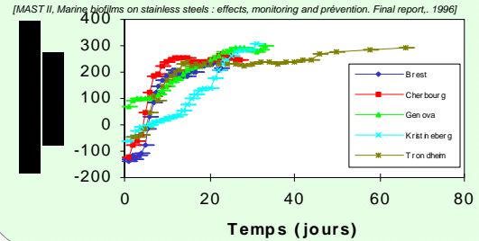
SEA WATER Free corrosion potential evolution of 254 SMO stainless steel coupons in natural seawaters
