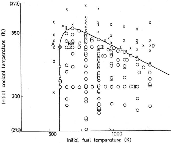
Figure 3: Fuel-coolant interaction zone for 1.2 \cdot 10^{-2} kg of tin dropped into water (0 indicates interaction, X indicates no interaction) (Figure 5 from [7])
