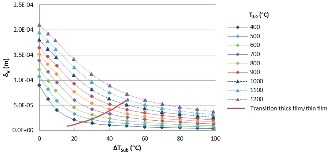
Figure 9: Variation of the vapor film thickness \delta_v as a function of the subcooling for different droplet temperatures ( D_s=14.6\text{mm} , U_\infty = 0.8 \text{ m}\cdot\text{s}^{-1} ) - "Thick film"/"thin film" transition line
