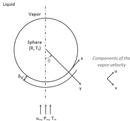
Figure 8: Coordinates system of the simplified film boiling model
