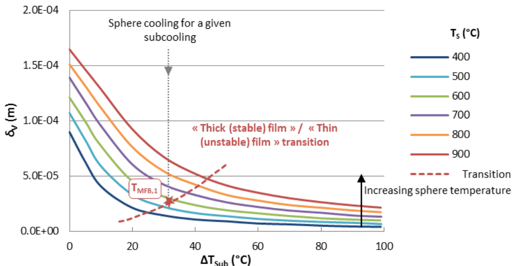
Figure 7: Simplified determination of the transition between the "stable" and "unstable" film boiling regimes Before using such a modeling for UO_2 -Na systems, for which no FCI zone (as the Reynolds et al. one) is available, we will apply it to the Reynolds experiment.
