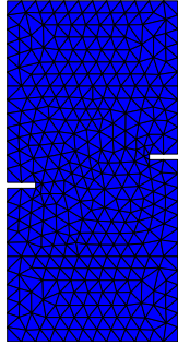
(a) Mesh with 672 elements.
