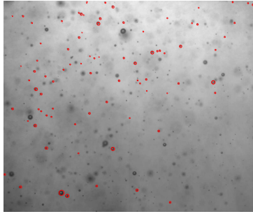
(a) One picture of the clouds and the bubbles detected. The void fraction is estimated to be around 1.4 \times 10^{-4}
