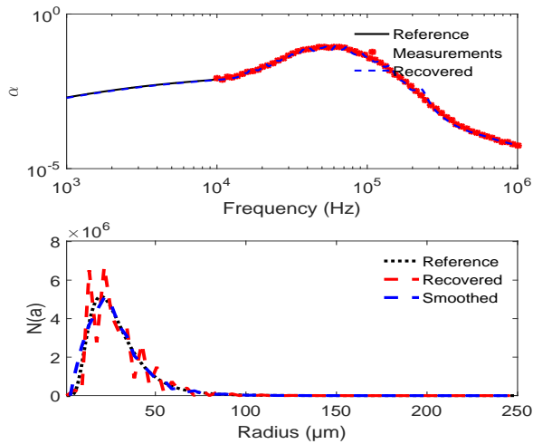
(b) Medium bandwidth: 10kHz \leq f \leq 1MHz \lambda = 2.10^{-5} \tau_{inv} = 7, 3.10^{-6}
