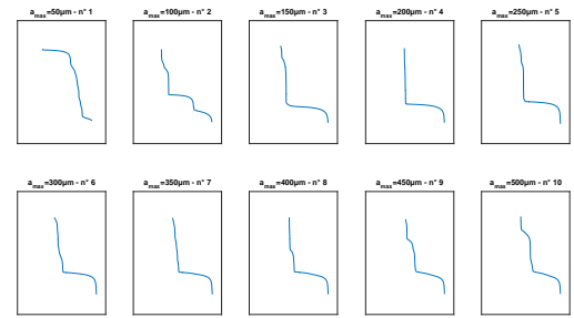
Figure 10: Several L-curves for different maximum radius of integration R_{\max} .
