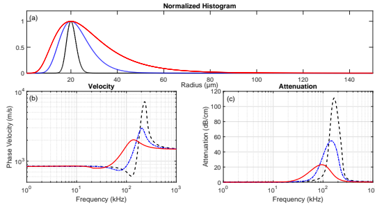
Figure 2: Impact of the bubble size distribution (a) on velocity (b) and attenuation (c). The distribution is log-normal (eq. (15)) with a scale parameter varying of 0.1 (black); 0.3 (blue) and 0.5 (red). \tau = 10^{-4}
