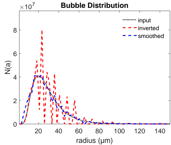
(a) \lambda = 0
