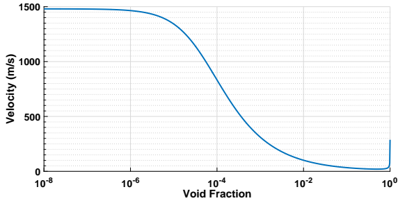
Figure 1: Velocity as a function of void fraction for air bubbles in water calculated using equation (10)
