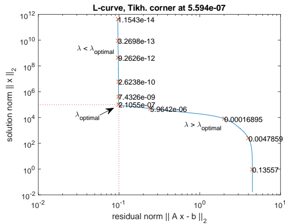
Figure 3: Example of a L-curve used for the determination of the optimal regularization parameter. Matlab script written by Hansen [22]
