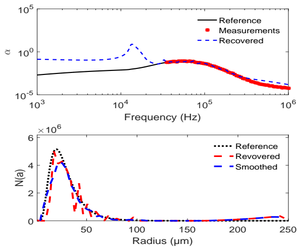
(c) Narrow bandwidth: 30kHz \leq f \leq 1MHz \lambda = 0.03 \tau_{inv} = 2.10^{-4}
