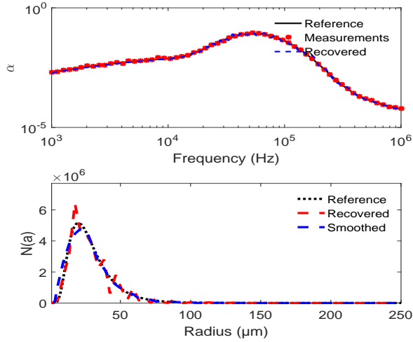
(a) Large bandwidth: 1kHz \leq f \leq 1MHz \lambda = 1.10^{-5} \tau_{inv} = 7, 3.10^{-6}
