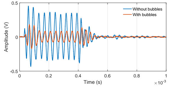
Figure 7: Example of bursts received. f = 13kHz
