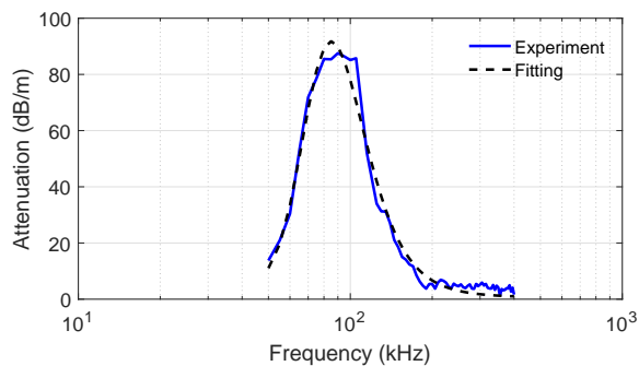
Figure 9: Experimental attenuation and attenuation obtained by fitting
