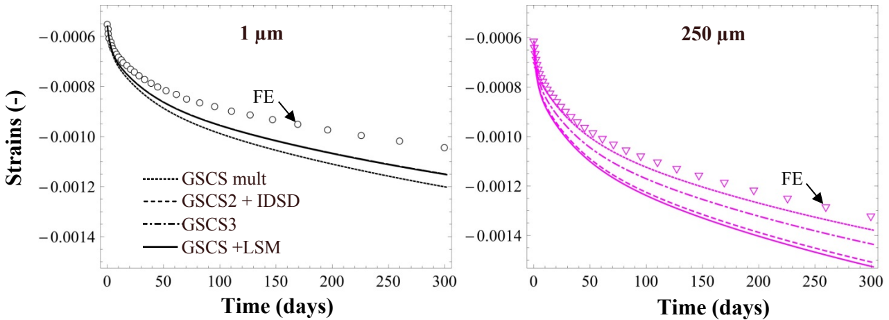
Figure 12. Longitudinal creep strains obtained numerically (symbols) and analytically with the GSCS2 + LSM (continuous lines), the GSCS2 + IDSD (dashed lines), the GSCS2 mul (dotted lines) and the GSCS3 (dot-dash lines) for interface thicknesses of 1 (black, left) and 250 (pink, right) \mu\text{m} .
