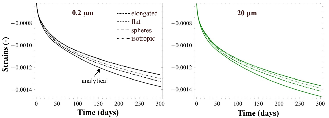
931 Figure 8. Analytical (GSCS) and numerical macroscopic longitudinal strain for interface thickness of 0.2 932 (left) and 20 μm (right) obtained for different aggregate shapes in the case of the 40% aggregate 933 mesostructure. The numerical results for the elongated and flat aggregates are almost superposed. 934
