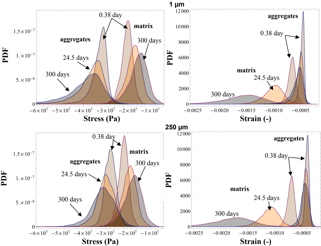
Figure 14. FE Probability Distribution Function for the average longitudinal stress (left) and strain (right) in both matrix subvolumes and aggregates for the 1 μm (top) and 250 μm (bottom) interface thickness and at 0.38, 24.5 and 300 days.
