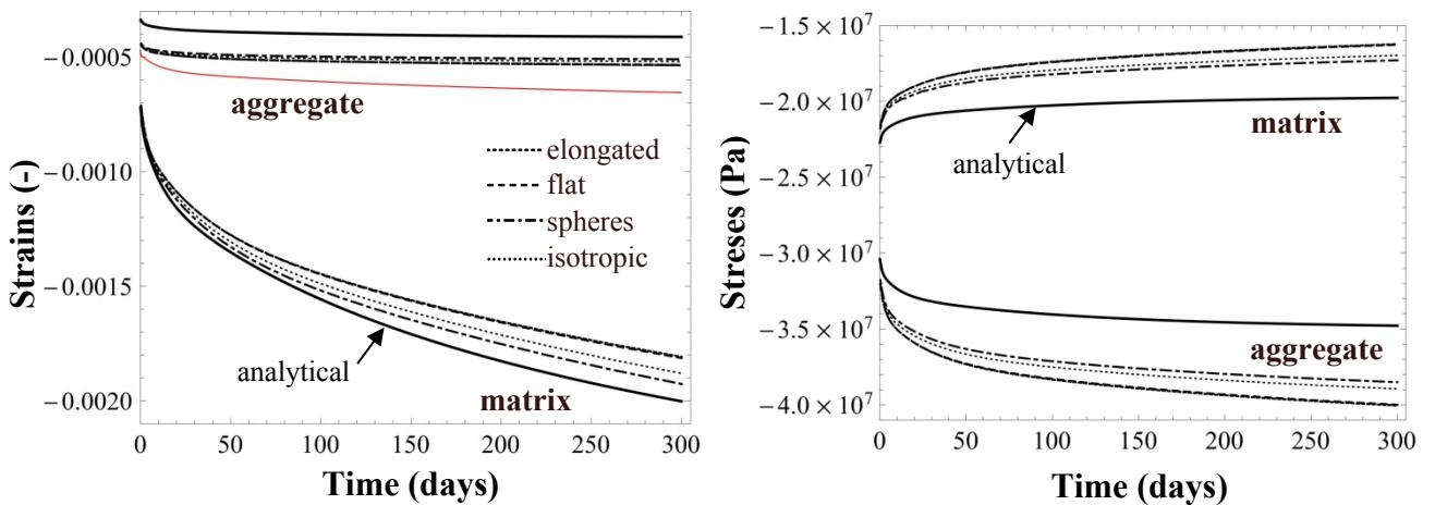
950 Figure 9. Analytical (GSCS) and numerical longitudinal strain (left) and stress (right) in both matrix and 951 inclusion phases for interface thickness of 20 μm obtained for different aggregate shapes in the case of the 952 40% aggregate mesostructure. The red plain curve on the left corresponds to the analytical strain of the 953 composite aggregate (i.e. aggregate + interface). The numerical results for the elongated and flat aggregates 954 are almost superposed. 955
