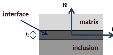
348 349 350 351 352 353 354 Figure 2. Schematic representation of a thin interface between an inclusion and the matrix. 355 356 357 358 359 360
