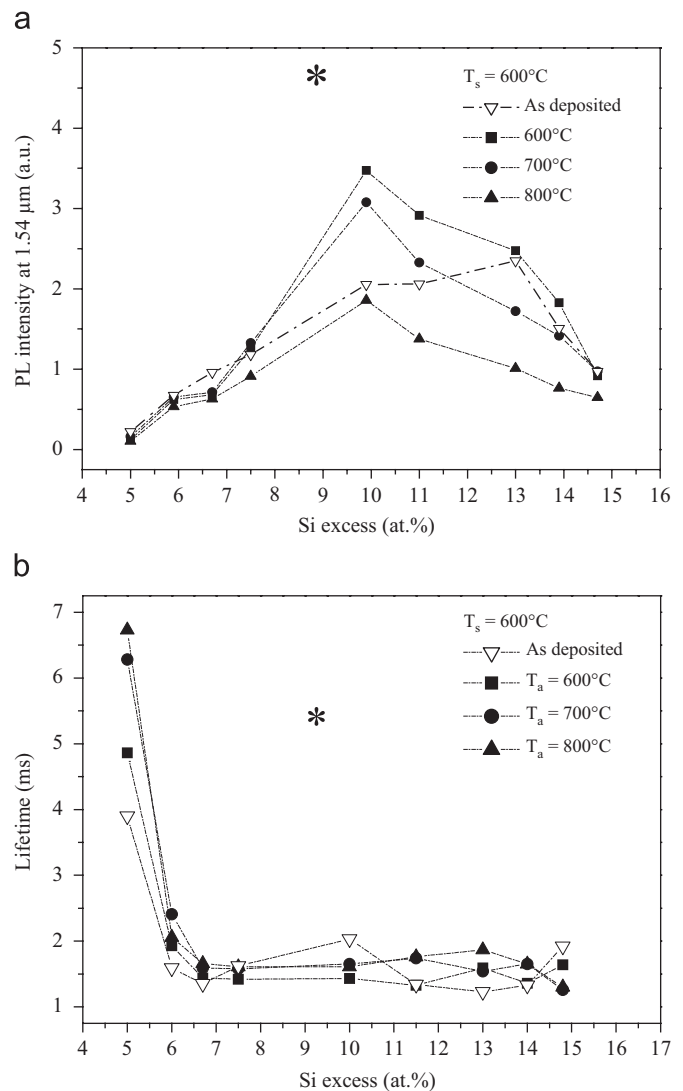
Fig. 4. (a): The PL intensity at 1.54 μm as a function of the Si excess with non-resonant excitation ( \lambda = 476 nm), for the as-deposited and annealed samples at the indicated temperature. (b): Evolution of the emission lifetime for the samples of Fig. 4(a) against the Si excess. The two experimental points labeled by (*) for the PL intensity and lifetime were obtained for the sample containing lower Er content than those of the main plots ( 3.5 \times 10^{20} vs. 10^{21} at cm -3 ) and a Si excess of about 9 at%.
