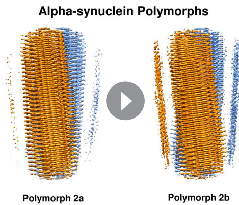
Video 1. Comparison of cryo-EM maps of \alpha -Syn fibril polymorphs. Cryo-EM reconstructions of \alpha -Syn fibrils at 3.1 Å (polymorph 2a) and 3.5 Å (polymorph 2b) resolution detailing the interaction between two protofilaments (blue and orange) in each fibril, the 4.9 Å spacing between \beta -strands and the topology of \alpha -Syn monomers within a single protofilament. https://elifesciences.org/articles/48907#video1
