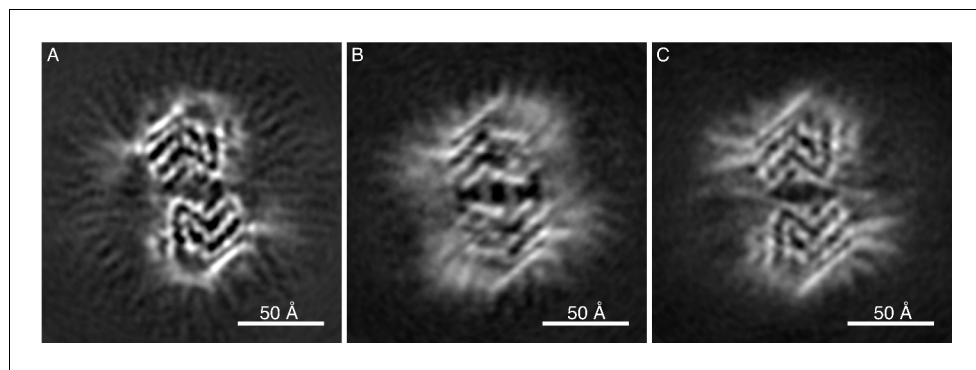
Figure 3. Cryo-EM cross-sections of fibrils, formed by E46K, p-S129 phosphorylated, and N-terminally acetylated \alpha -Syn protein. Fibrils formed by E46K mutant \alpha -Syn protein (A), Ser129 phosphorylated \alpha -Syn protein (B), and N-terminally acetylated \alpha -Syn protein (C) were analyzed by cryo-EM. Image processing did not allow reaching sufficient resolution for model building, but the cross-sections of the obtained 3D reconstructions are compatible with polymorph 2a for all three forms.
