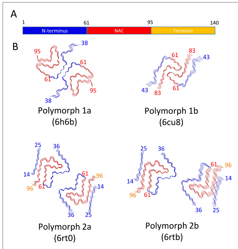
Figure 4. Schematic representation of \alpha -Syn polymorphs. (A) Diagram representing \alpha -Syn regions with the N-terminus in blue, the NAC region in red and the C-terminus in yellow. (B) Representation of \alpha -Syn fibril polymorphs 1a (PDB ID 6h6b; Guerrero-Ferreira et al., 2018 ), 1b (PDB ID 6cu8; Li et al., 2018a ), 2a (PDB ID 6rt0, this work), and 2b (PDB ID 6rtb, this work), highlighting the striking differences in protofilament folding in \alpha -Syn polymorphs 1a and 1b, compared to \alpha -Syn polymorphs 2a and 2b. The atomic models obtained by cryo-EM of \alpha -Syn polymorph 1a, polymorph 1b ( Li et al., 2018a ; Li et al., 2018b ) and \alpha -Syn polymorphs 2a and 2b (this work). Protein Data Bank (PDB) accession numbers are indicated.
