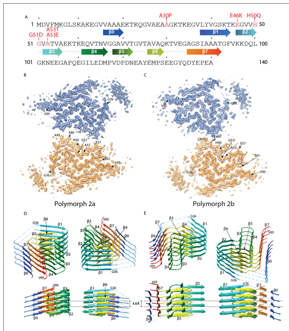
Figure 1. Cross-sections of the \alpha -Syn polymorph 2a and 2b cryo-EM structures. (A) Sequence of human \alpha -Syn with familial PD mutation sites indicated in red. \beta strands are indicated by arrows colored from blue to orange. Cryo-EM densities and atomic models of polymorph 2a (B) and polymorph 2b (C) of \alpha -Syn. Each cryo-EM map shows two protofilaments (blue and orange) forming a fibril. PD-associated mutations sites, and first and last residues of the NAC regions are indicated. (D and E) Rainbow rendering views of the secondary structure elements in five successive rungs of both polymorphs. A view perpendicular to the helical axis is shown to illustrate the height differences in a single \alpha -Syn fibril. Colors correspond to the arrows in the sequence displayed in panel (A). The online version of this article includes the following figure supplement(s) for figure 1:
