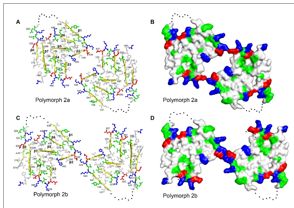
Figure 2. Structure and distribution of amino acids in the new \alpha -Syn fibril polymorphs. Amino acids are colored in blue for positively charged, in red for negatively charged, in green for polar (including glycine), and in white for hydrophobic residues. Even and odd numberings are given on one monomer each. (A and C) Backbone structure. (B and D) Surface view.
