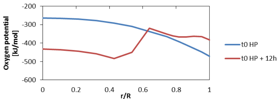
Fig. 9. Oxygen potential radial profile at mid-pellet plane at “t0 HP” and “t0 HP + 12h”.
