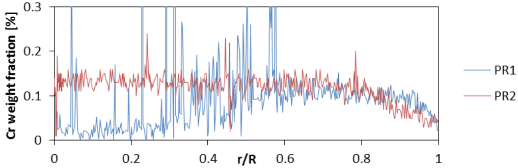
Fig. 5. EPMA measurements of chromium weight fraction in solid solution after PR1 and PR2.
