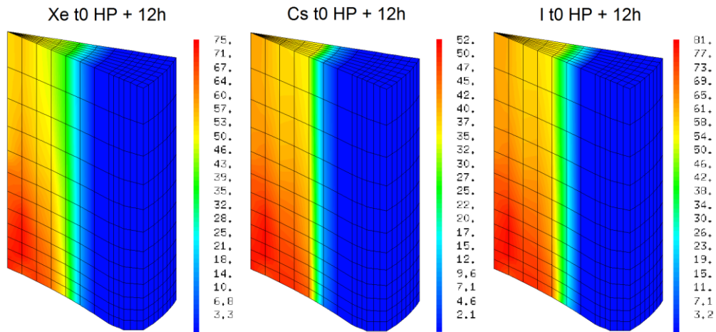
Fig. 15. Release of Xe, Cs and I at "t0 HP + 12h". Units - % of initial inventory.
