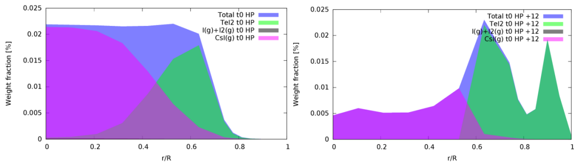
Fig. 14. Speciation of gaseous iodine at “t0 HP” and “t0 HP + 12h” along the inter-pellet plane.
