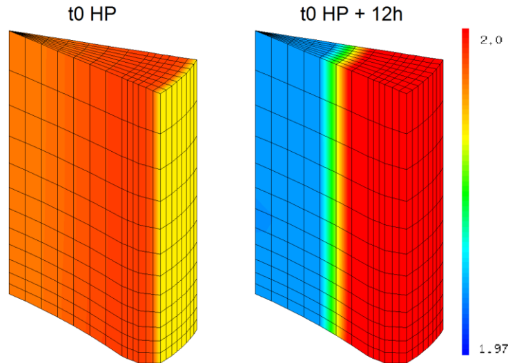
Fig. 7. O/M in the simulated fuel fragment at the beginning (left figure) and at the end (right figure) of the Holding Period. The top plane of this fragment is the mid-pellet plane and the bottom plane is the inter-pellet plane.
