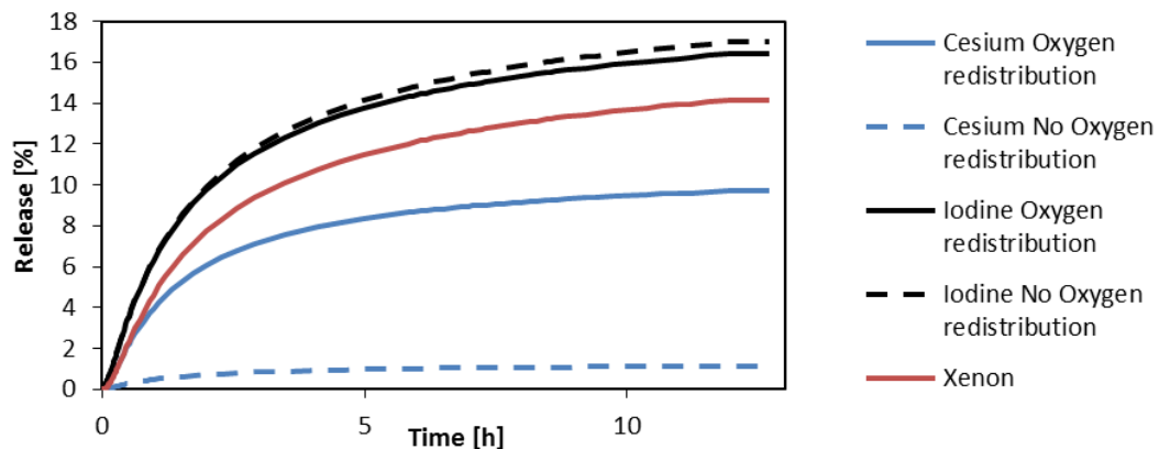
Fig. 17. Release of Cs, I and Xe in function of time. Solid lines – simulation with oxygen redistribution, dashed lines – simulation without oxygen redistribution. The graph starts at "t0".
