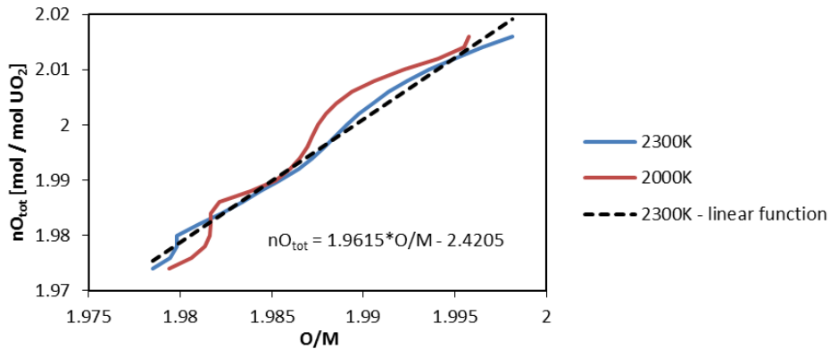
Fig. 6. Total Oxygen content n_{O}^{\text{tot}} in function of the O/M ratio at 2000 K and 2300 K. The equation describes the black line which is the linear approximation of the curve for 2300 K.
