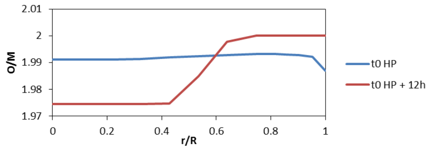
Fig. 8. O/M at “t0 HP” and “t0 HP + 12h” in function of relative radius.
