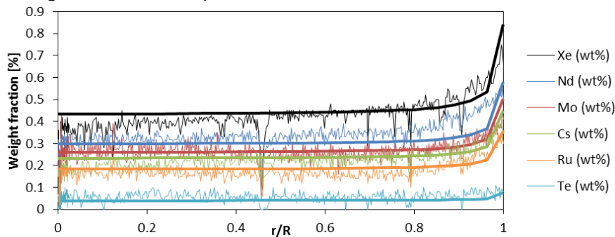
Fig. 2. Comparison of calculated weight fractions of FPs (thick lines) with EPMA measurements (thin lines) after the PR2 test (see Tab. 2).
