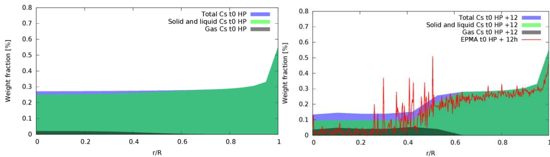
Fig. 13. Calculated speciation of caesium at “t0 HP” and “t0 HP + 12h” along the inter-pellet plane compared to EPMA measurements after PR1 test.
