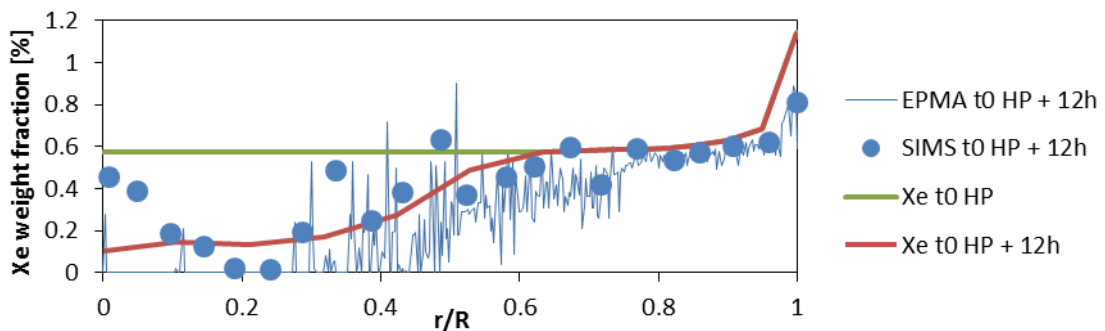
Fig. 16. Total (dissolved within grains, in intra- and inter-granular bubbles and in inter-granular pores) Xe weight fraction at the beginning and the end of the holding period compared to EPMA and SIMS measurements.
