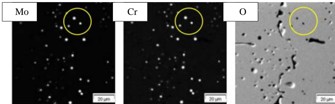
Fig. 10. X-ray images of Mo, Cr and O at the centre of the pellet [3] after PR1 test.
