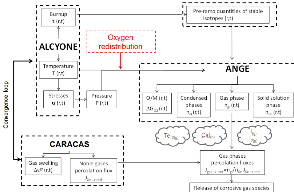
Fig. 3. Schematic representation of the coupling between the fuel performance code ALCYONE, the thermo-chemical solver ANGE, the fission gas release model CARACAS and the oxygen redistribution model.
