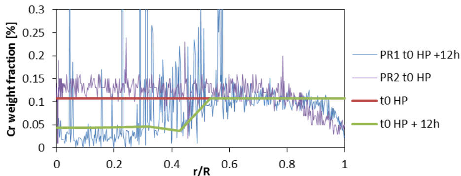
Fig. 11. Calculated Cr weight fraction evolution during the Holding Period of PR1 test compared to EPMA measurements after PR1 and PR2 tests.
