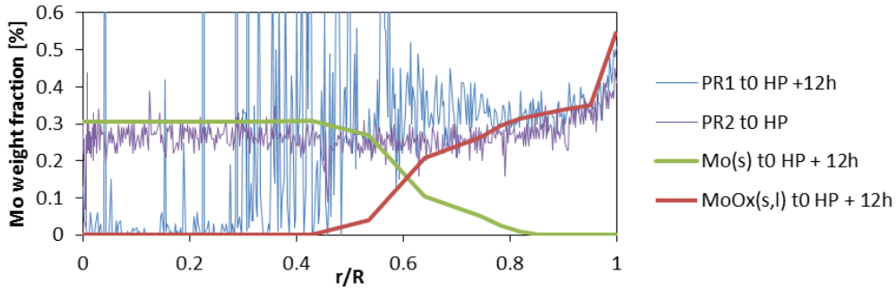
Fig. 12. Calculated molybdenum oxides \text{MoO}_{x(s,l)} and metallic molybdenum \text{Mo}_{(s)} weight fraction evolution during the Holding Period of PR1 tests compared to EPMA measurements after PR1 and PR2 tests. PR2 rodlet has a slightly lower burnup than PR1 rodlet so the Mo weight fraction is lower on average.
