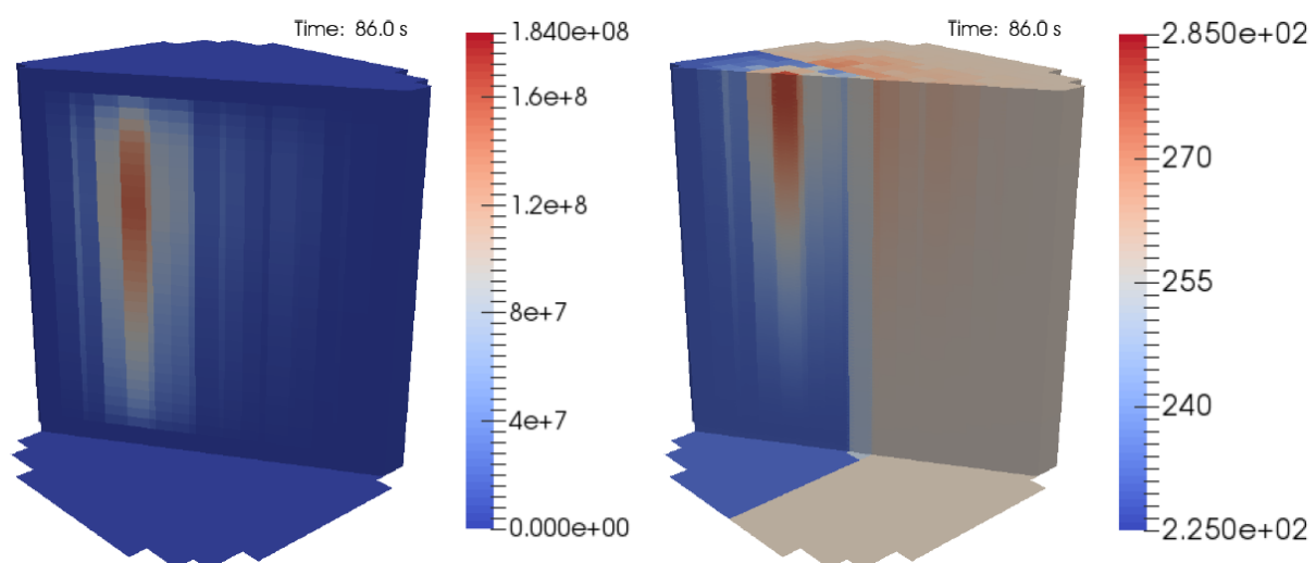
Fig. 5 Distribution of power density ( \text{MW/m}^3 , left) and coolant temperature ( ^{\circ}\text{C} , right) at 86 s after the initiation of the MSLB event.
