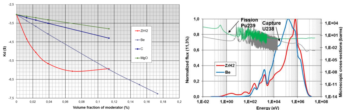
Figure 1 : Doppler constant depending on volume fraction of 4 different moderators inserted (left) - Flux spectrum (ZrH 2 , Be) and microscopic cross sections of fission ( ^{239}\text{Pu} ) and capture ( ^{238}\text{U} ) (right)
