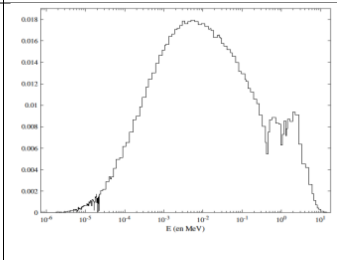
Figure 5. Epithermal configuration - Neutron spectrum in the central channel
