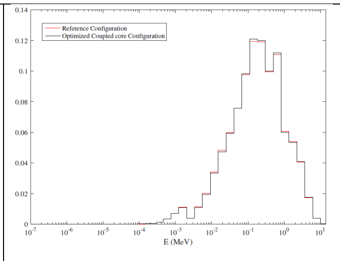
Figure 3. Fast-thermal configuration - Neutron spectrum in the central channel
