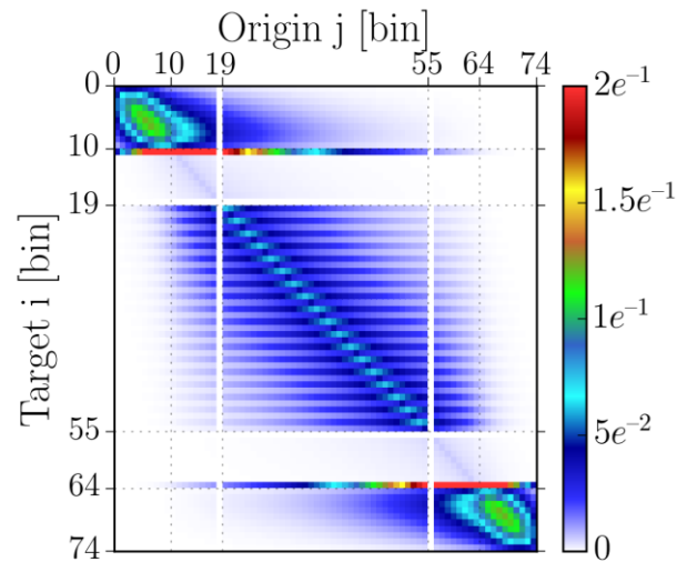
Figure 11: \underline{G}_{\chi_p \nu_d} “prompt-to-delayed” fission matrix
