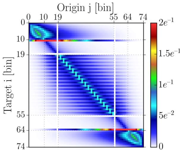
Figure 10: \underline{G}_{\chi_p \nu_p} “prompt-to-prompt” fission matrix
