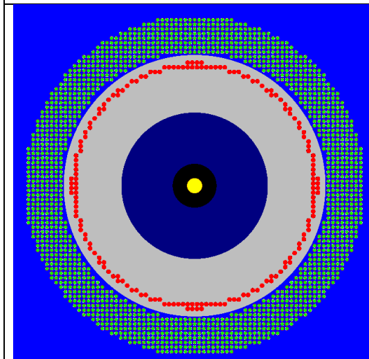
Figure 4. Epi-thermal configuration - TRIPOLI-4® model in X-Y plane
