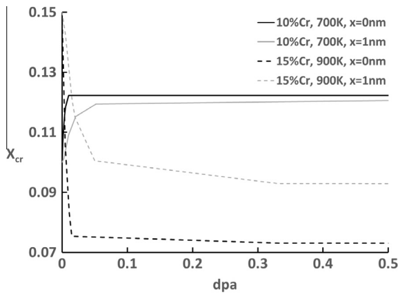
Fig. 9. Concentration of Cr at sink ( x = 0 nm, black line) and at a distance of 1 nm from the sink ( x = 1 nm, grey line) as a function of dose in Fe-15%Cr at 900 K (dotted line) and in Fe-10%Cr at 700 K (full line), calculated using PF.
