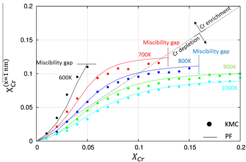
Fig. 10. Atomic fraction of Cr measured at a distance x = 1 nm from the planar sink, X_{Cr}^{(x=1 \text{ nm})} , as a function of the mean Cr fraction and temperature, calculated using AKMC (symbols) and PF (lines). Calculations are performed at K_0 = 10^{-5} \text{ dpa s}^{-1} and \rho = 10^7 \text{ m}^{-1} . Vertical and horizontal dashed lines correspond to the limit of the miscibility gap. The dashed line X_{Cr}^{(x=1 \text{ nm})} = X_{Cr} represents the limit between Cr depletion and Cr enrichment.
