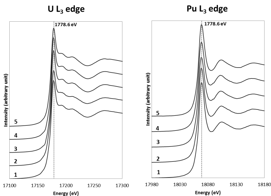
Figure S1. Normalized XANES at uranium (left) and plutonium (right) L 3 edge for (1) M-DBBA-S (solid sample) (2) M-DBBA-L (in toluene) (3) M-DEHBA (4) M-DEHDMBA and (5) M-DEHiBA (M = U, Pu)
