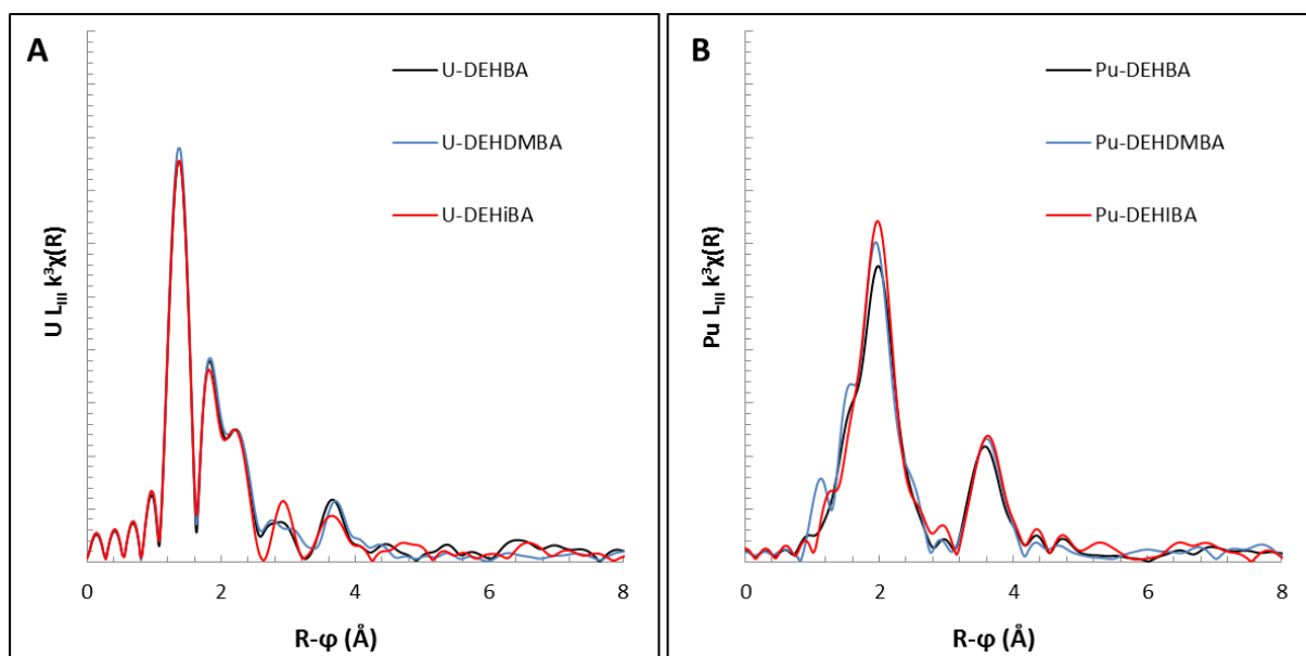
Figure S2. Experimental FT's modulus part at uranium (A) and plutonium (B) L 3 edge for M-DEHBA, M-DEHDMBA and M-DEHiBA (M = U, Pu)
