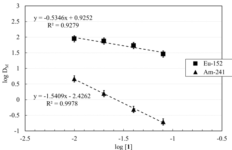
Figure S12 Distribution ratios for Am(III) and Eu(III) as a function of [ 1 ]. Organic phase : 0.2 M TODGA in kerosene + 5 v/v% 1-octanol loaded with 241 Am and 152 Eu and scrubbed with 0.5 M HNO 3 ; Aqueous phase : 1 in 0.44 M HNO 3 .
