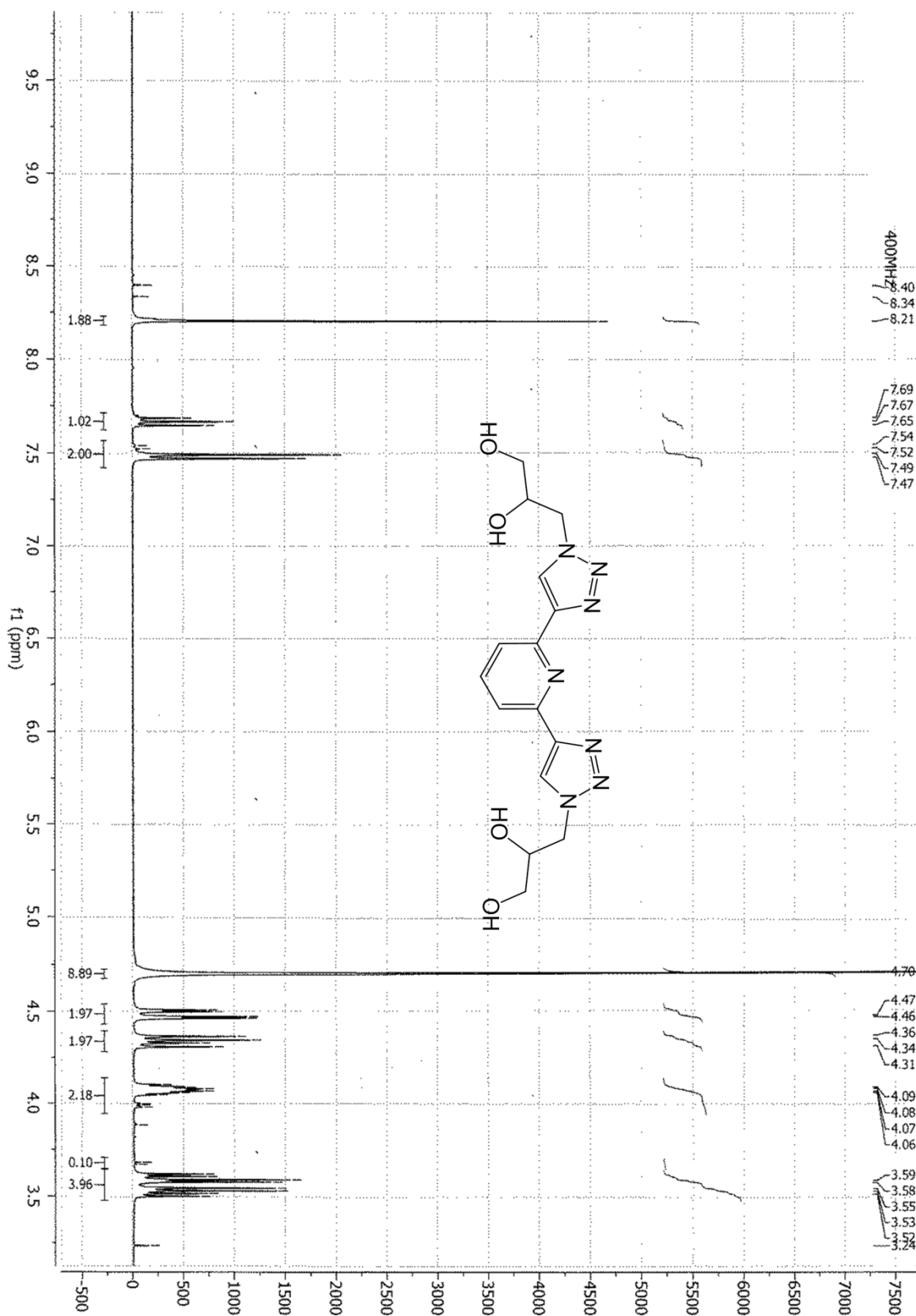
Figure S3 1 H NMR spectrum (D 2 O, 400MHz, 300K) of compound 2
