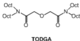
Figure S9 Molecular structure of N,N,N',N'-tetraoctyl diglycolamide (TODGA).
