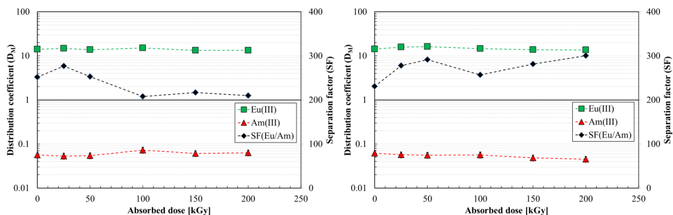
Figure S10 Distribution coefficients and separation factors for ligand 1 (left) and 2 (right) stripping solutions as a function of the absorbed dose. Organic phase: 0.2 M TODGA in kerosene/1-octanol (95/5 v/v) loaded with GANEX FEED; Aqueous phase: irradiated 0.08 M of ligand 1 or 0.15 M of ligand 2 , [\text{HNO}_3]_{\text{in}}=0.44 M (dose rate = 2.5 kGy/h).
