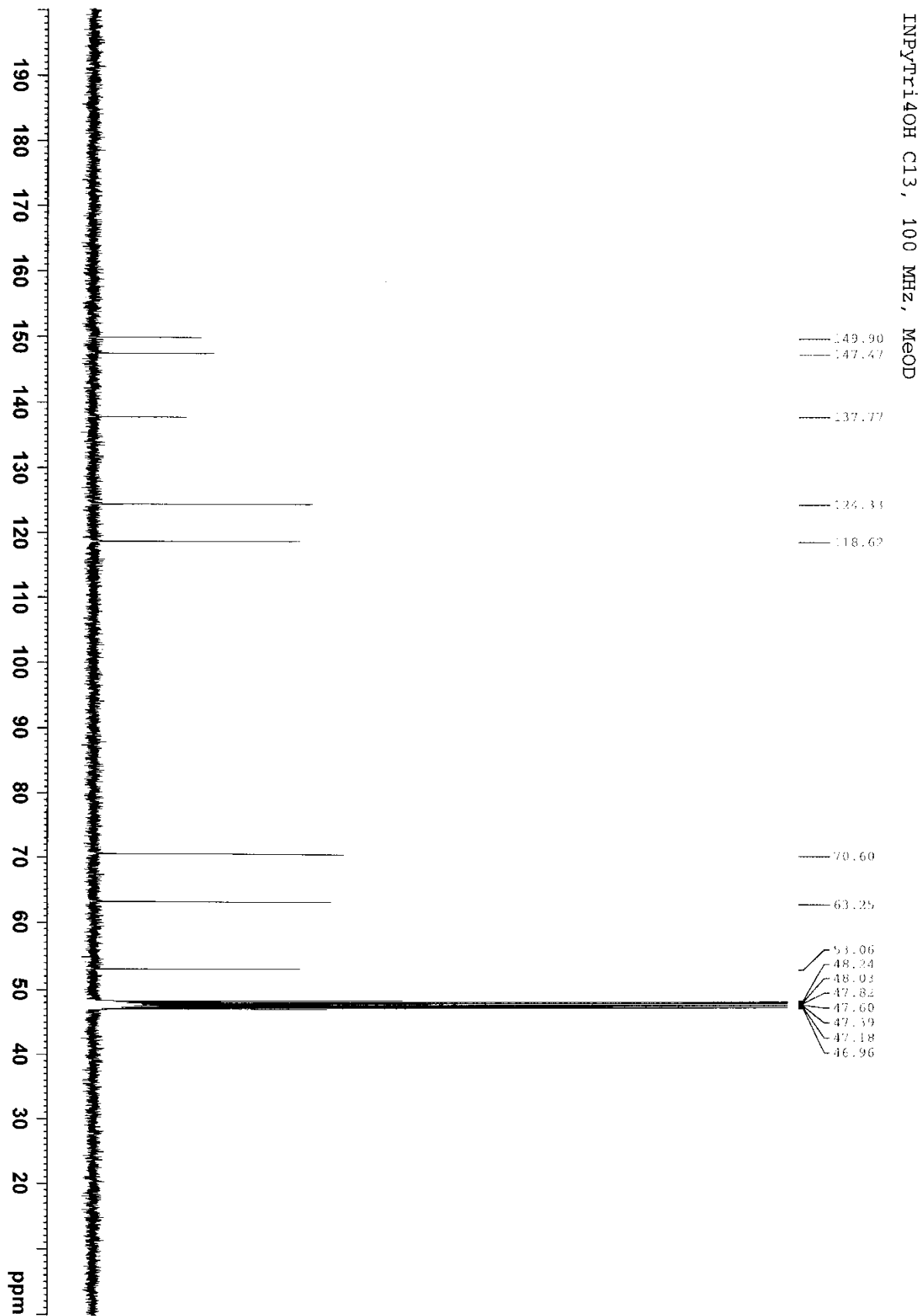
Figure S4 ^{13}\text{C} NMR spectrum (MeOD, 100MHz, 300K) of compound 2
