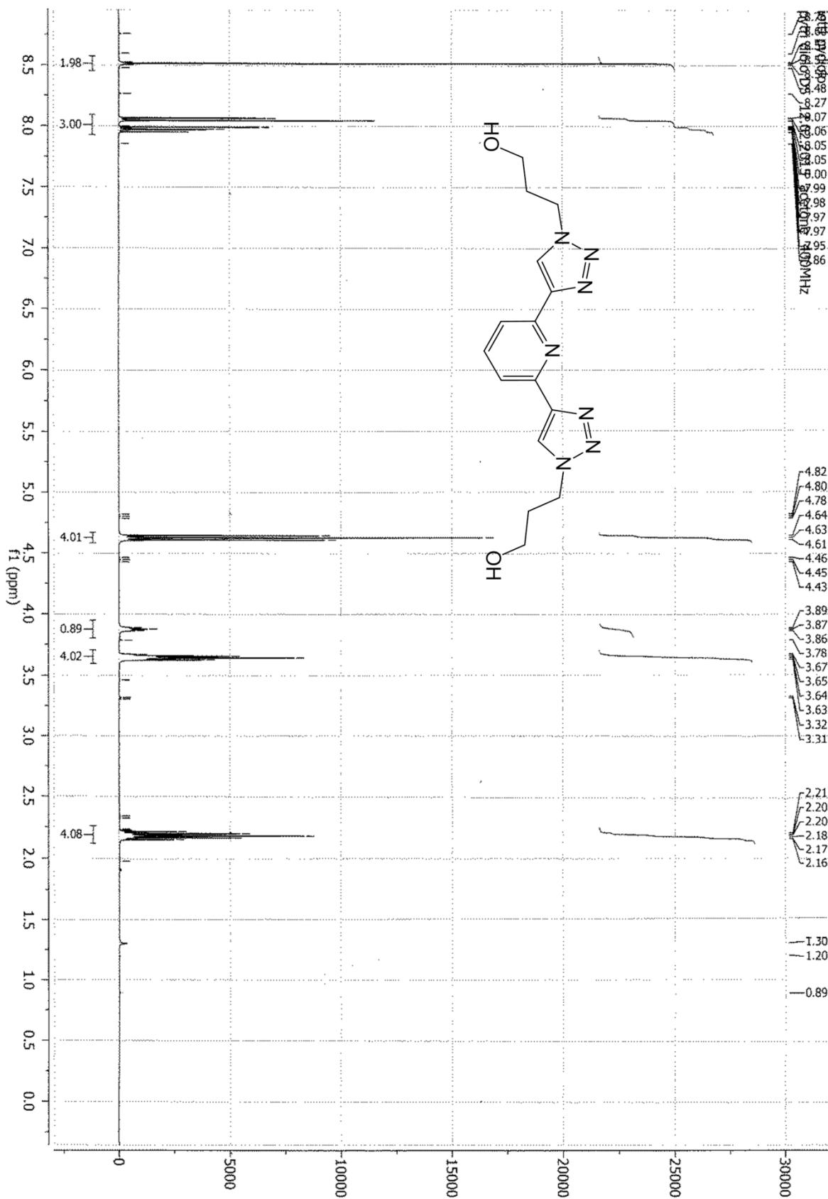
Figure S1 1 H NMR spectrum (Acetone-D 6 , 400MHz, 300K) of compound 1
