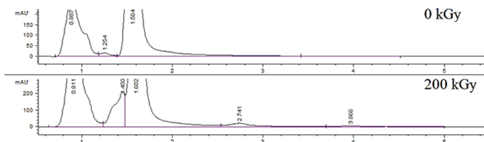
Figure S11 HPLC chromatograms of 1 solutions in 0.44 M \text{HNO}_3 irradiated up to 200 kGy (2.5 kGy/h).
