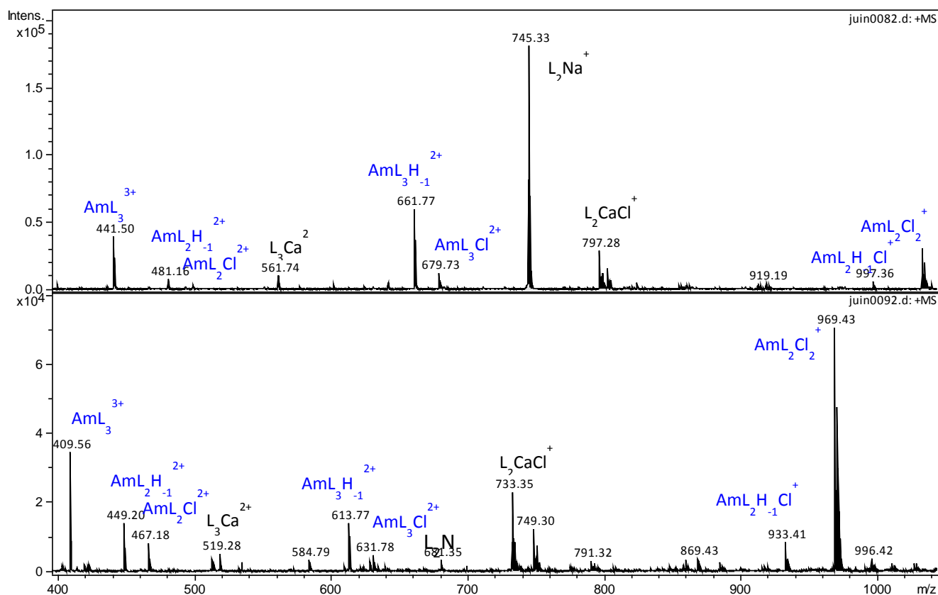
Figure S133: ESI-MS spectra of Am(III) ligand species in MeOH/H 2 O 75:25 (v/v). c_{\text{ligand}}/c_{\text{Eu}} = 10 . Zoom in the 400-1050 m/z. Top: Am-2 ligand solution and bottom Am-1 ligand solution.
