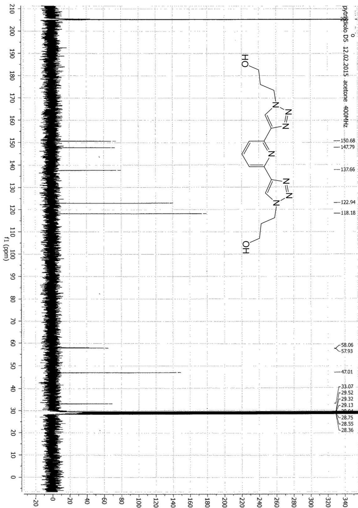
Figure S2 ^{13}\text{C} NMR spectrum (Acetone- \text{D}_6 , 100MHz, 300K) of compound 1
