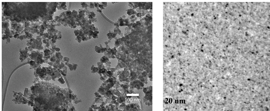
Figure 4: TEM of Cu-HCF Bulk particles (left) and templated (right). Average particles size is 20 \text{ nm} \pm 5 \text{ nm} and 15 \text{ nm} \pm 5 \text{ nm} respectively
