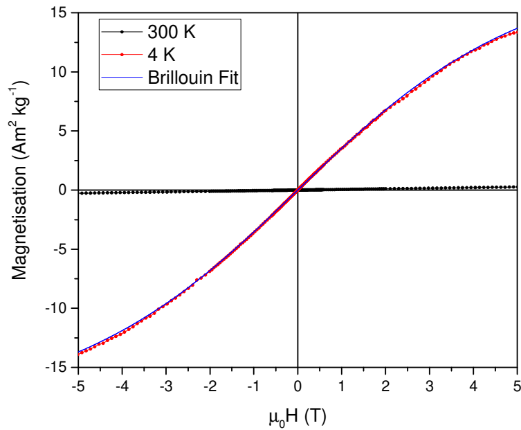
Figure 9: Magnetisation data of Cu-HCF aggregated particles at 300 K and 4 K
