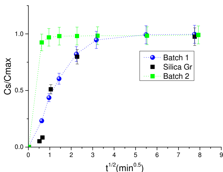
Figure 5: Cs sorption spectrum of batch 1 (no magnet, physical stirring) (blue circle), batch 2 (magnet, physical stirring) (green square) and Gr (silica grain) (black squares). Data is displayed as % Cs sorbed ( C_s/C_{max} where C_s is concentration of Cs at time t and C_{max} is total Cs exchanged) against the square root of time.
